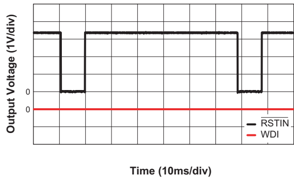
Watchdog Timer (WDI = 0V)
