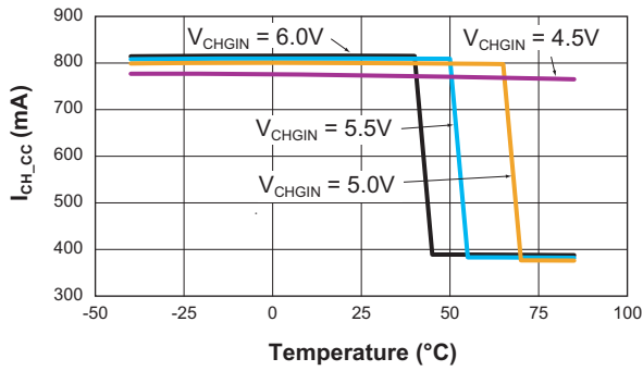
www.datasheet4u.com Constant Current Mode Charge Current vs. Temperature ( V_{BAT} = 3.6V ; R_{ISET} = 1.24k\Omega )
