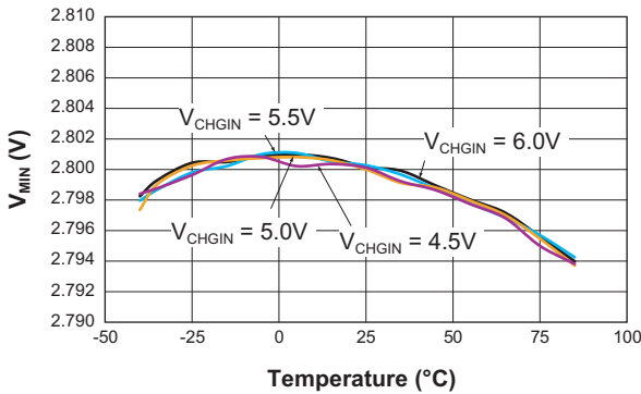
Preconditioning Threshold Voltage vs. Temperature www.datasheet4u.com
