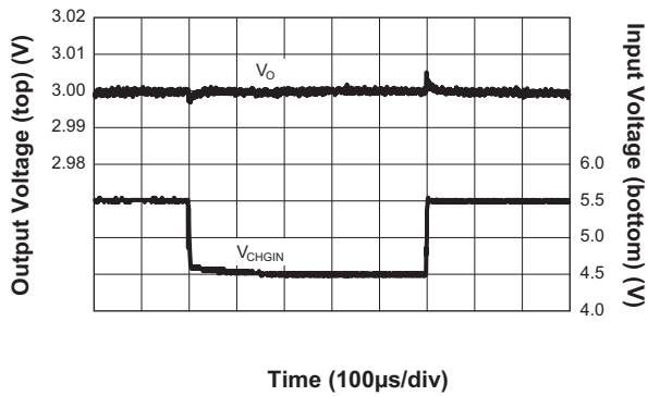
Line Transient Response LDO1 ( V_{CHGIN} = 4.5V to 5.5V ; I_{OUT} = 300mA ; V_{OUT} = 3V )
