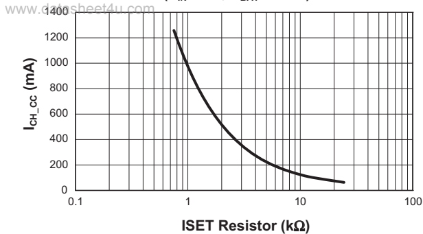
Figure 5: Constant Current Mode Charge I_{CH,CC} Setting vs. I_{SET} Resistor and I_{SET} Voltage vs. Battery Voltage.
