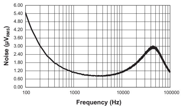
LDO Output Voltage Noise
