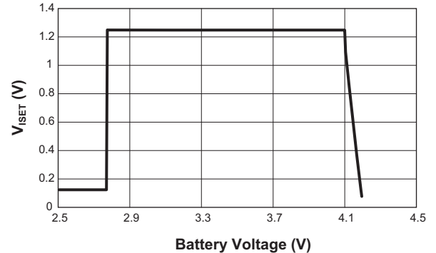
Figure 5: Constant Current Mode Charge I_{CH,CC} Setting vs. I_{SET} Resistor and I_{SET} Voltage vs. Battery Voltage.
