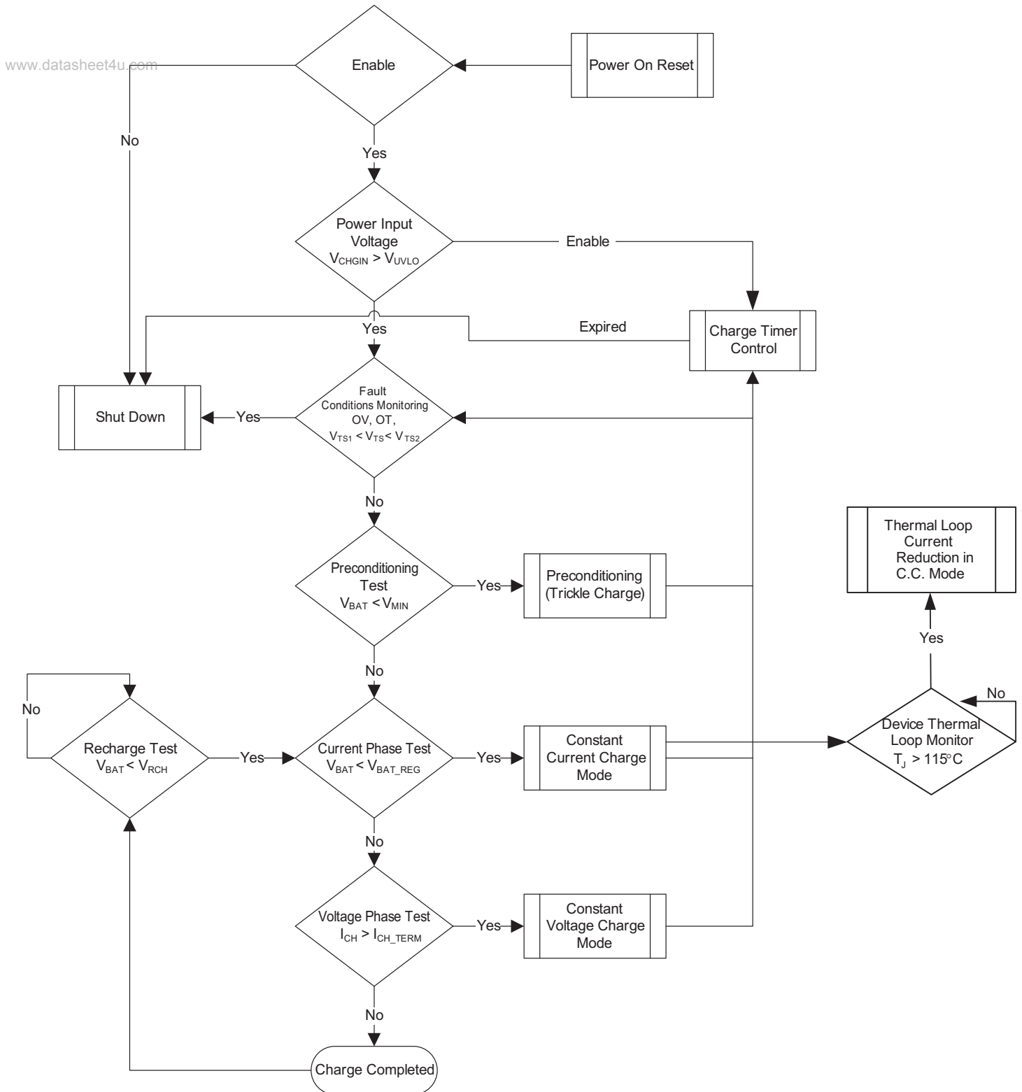
Figure 4: System Operation Flow Chart for the Battery Charger.
