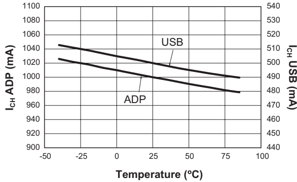
Fast Charge Current vs. Temperature ( R_{SETADP} = 8.06k\Omega ; R_{SETUSB} = 8.06k\Omega )
