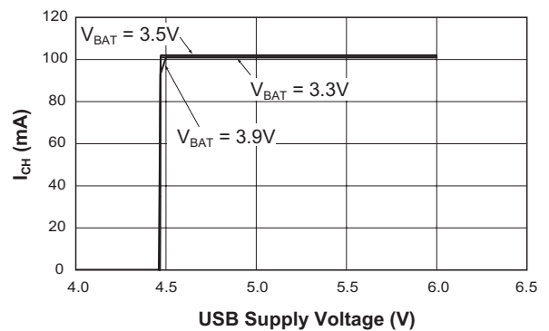
Fast Charge Current vs. USB Supply Voltage ( R_{SETUSB} = 42.4k\Omega )
