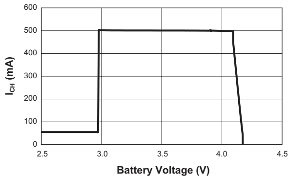
USB Charging Current vs. Battery Voltage ( R_{SETUSB} = 8.06k\Omega )
