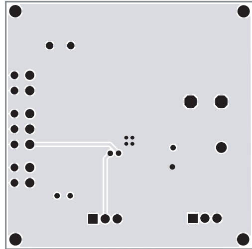
Figure 6: AAT3689 Evaluation Board Solder Side Layout.
