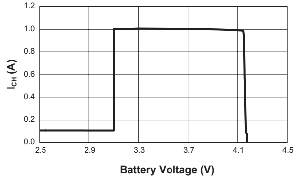
Adapter Charging Current vs. Battery Voltage ( R_{SETADP} = 8.06k\Omega )
