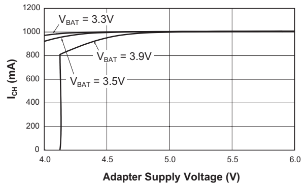
Fast Charge Current vs. Adapter Supply Voltage ( R_{SETADP} = 8.06k\Omega )
