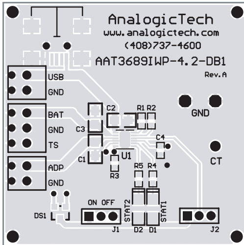
Figure 5: AAT3689 Evaluation Board Component Side Layout.
