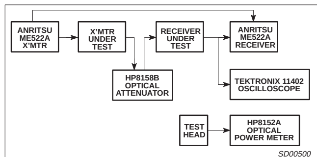
Figure 1. Test Set-Up
