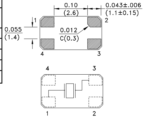
TOP VIEW Recommended land pattern
