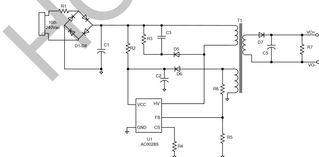
Typical application of AC0028S for RCC replace (Output: 5V/2.0A)
