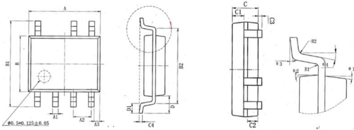
SOP7 Package
