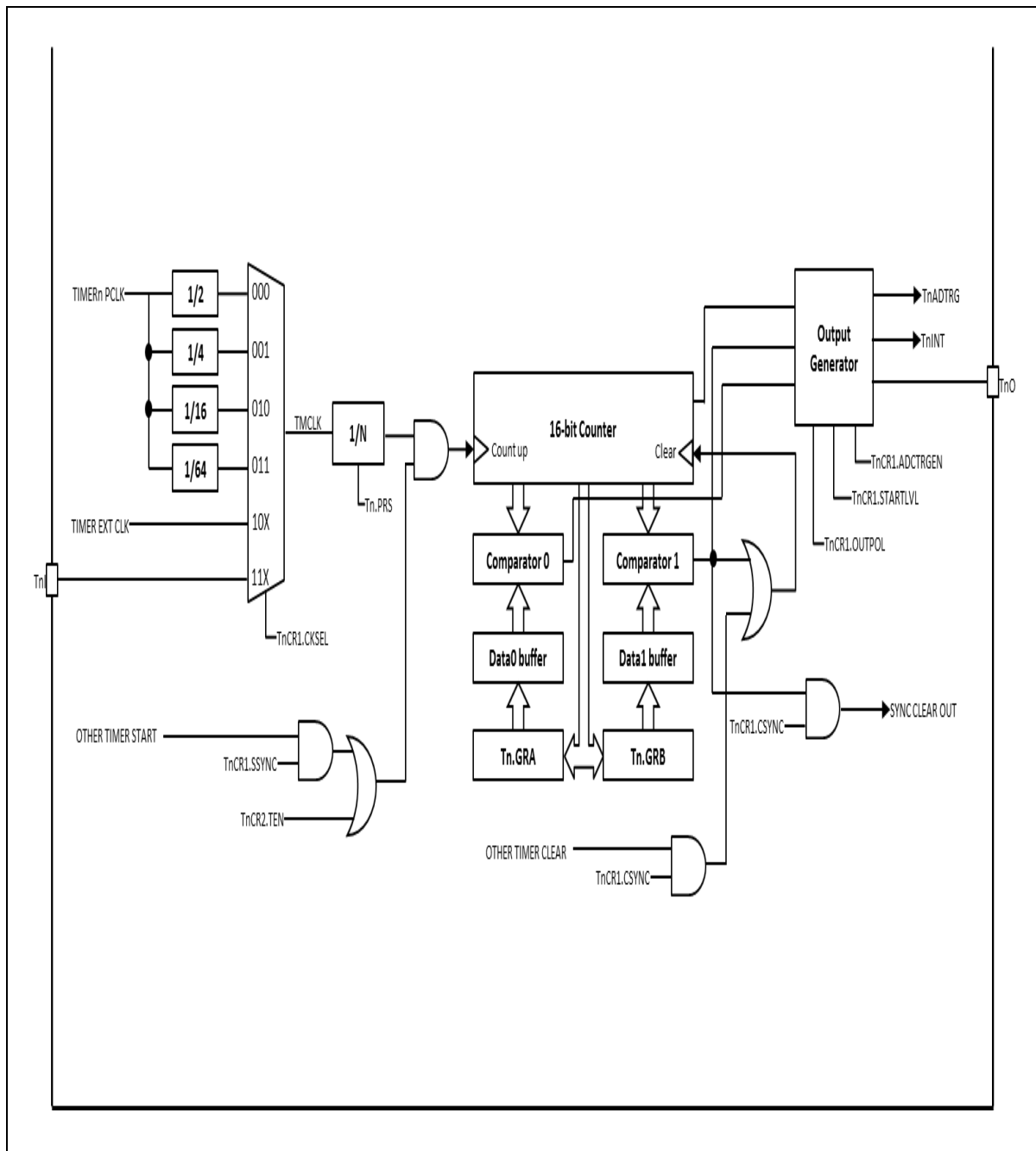
Figure 23. 16-bit Timer Block Diagram
