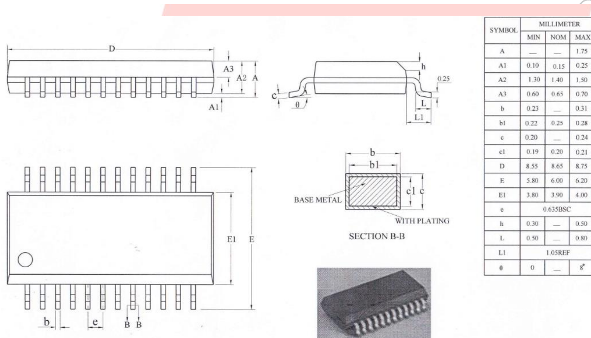
Figure 3-1. AC6965A Package
