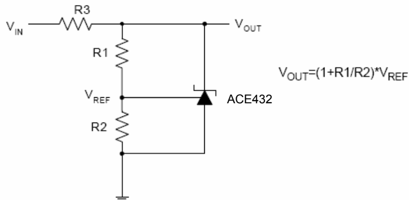
Figure 13. Shunt Regulator
