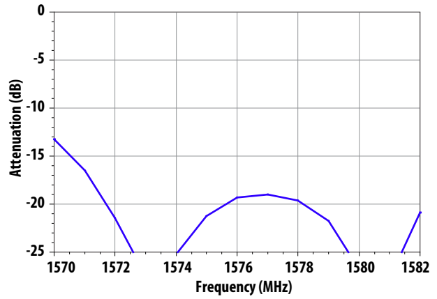
Figure 30. GPS Port Return Loss (Dual Antenna, Note1).
