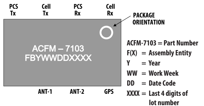
Figure 51. Package Marking
