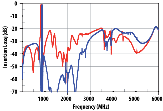
Figure 20. Cellular Tx-Ant and Ant-Rx Wideband Insertion Loss.
