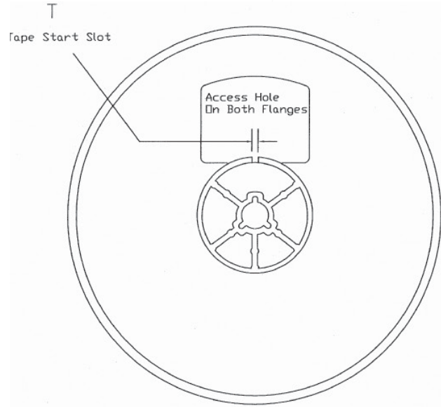
Figure 43. Reel Drawing
