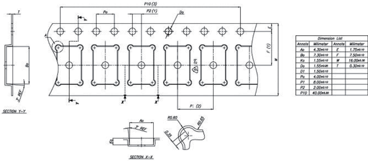
Figure 41. SMT Tape Packing
