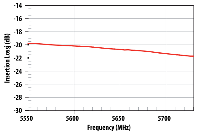
Figure 13. PCS Ant-Tx Rejection at Tx Third Harmonic.
