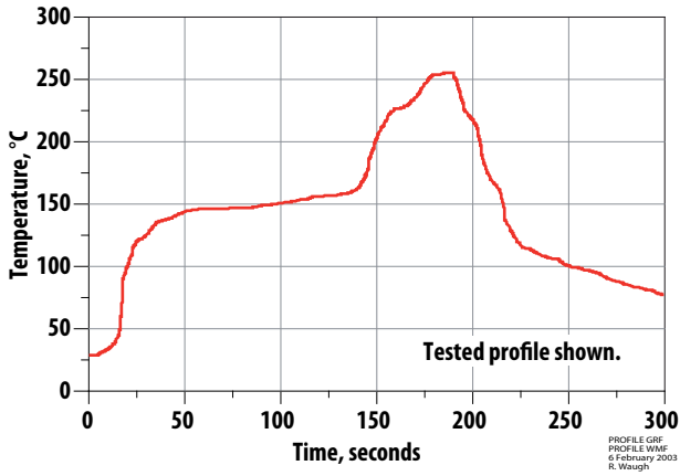
Figure 39. Verified SMT Solder Profile.
