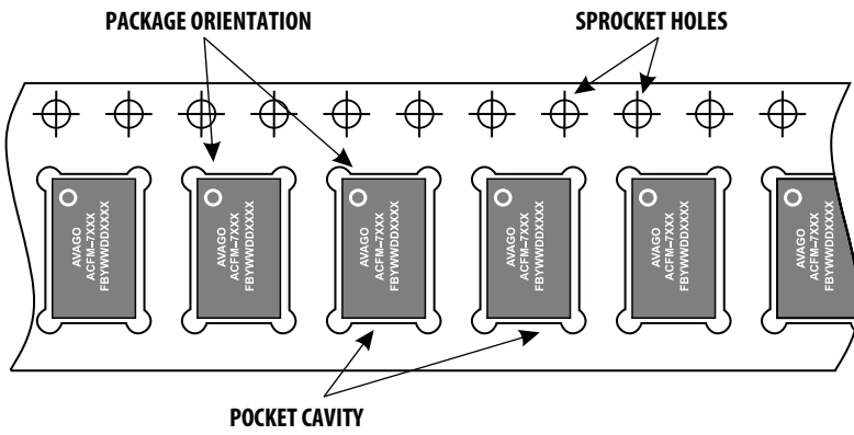
Figure 42. Orientation in Tape
