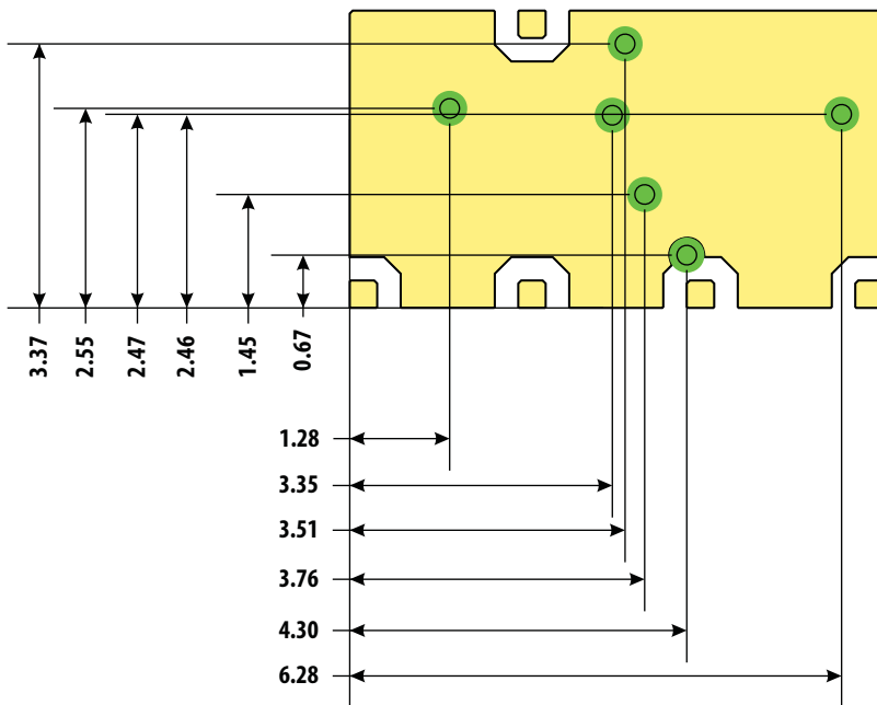
Figure 29. Locations of Non-Ground (Signal) Vias (bottom view).
