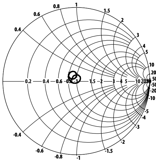
Figure 19. Ant Port Impedance in Cell Tx Band (824–849 MHz).
