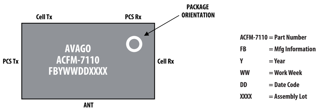
Figure 22. Package Marking
