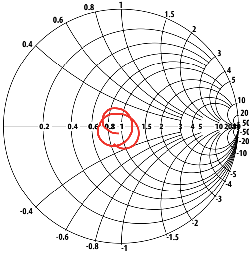
Figure 17. Cell Tx Port Impedance in Tx Band (824–849 MHz).
