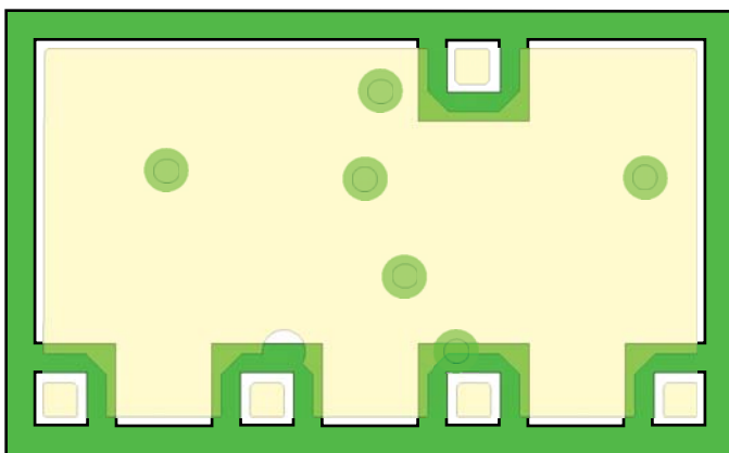
Figure 48. Solder Mask Superposed on ACFM-7325 Bottom Metal Pattern. (top view)
