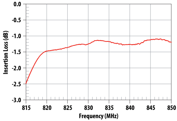
Figure 14. Cellular Tx Insertion Loss.
