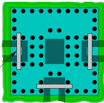
Shorting pin, soldered to in/out pad and to ground on both sides, three places.
