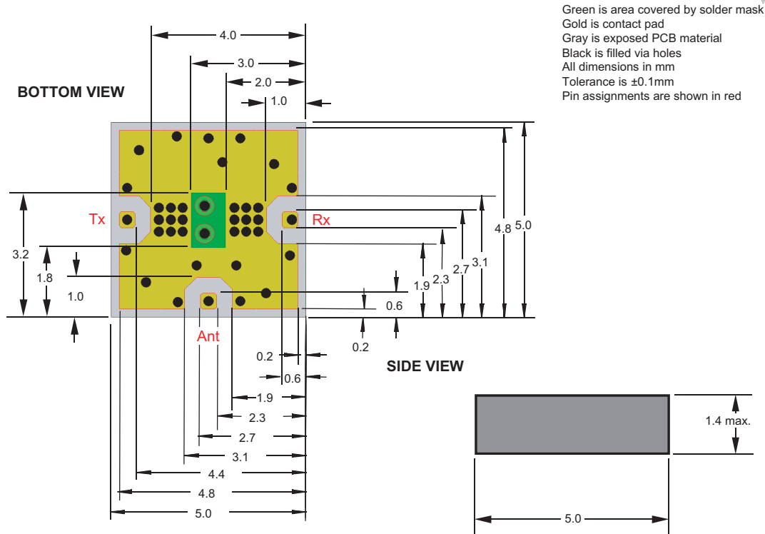
Figure 19. Outline drawing.
