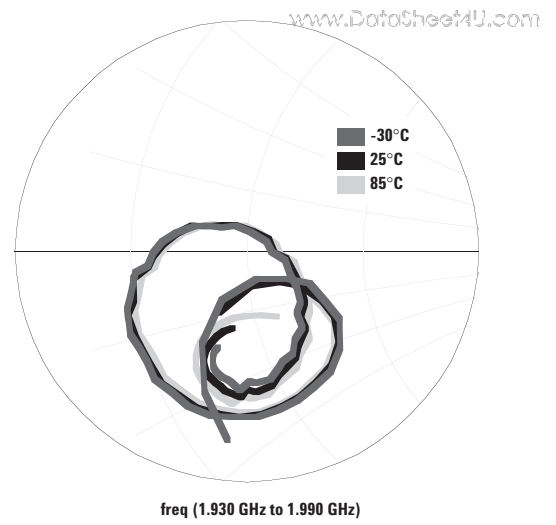
Figure 9. Rx port impedance (8 dB circle).
