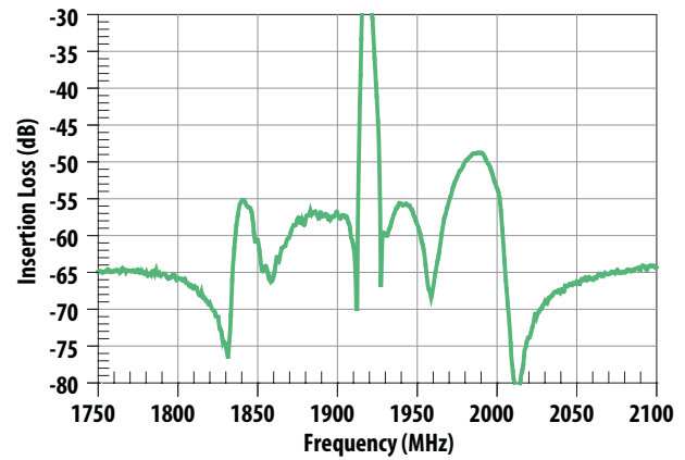
Figure 4. Tx-Rx Isolation.
