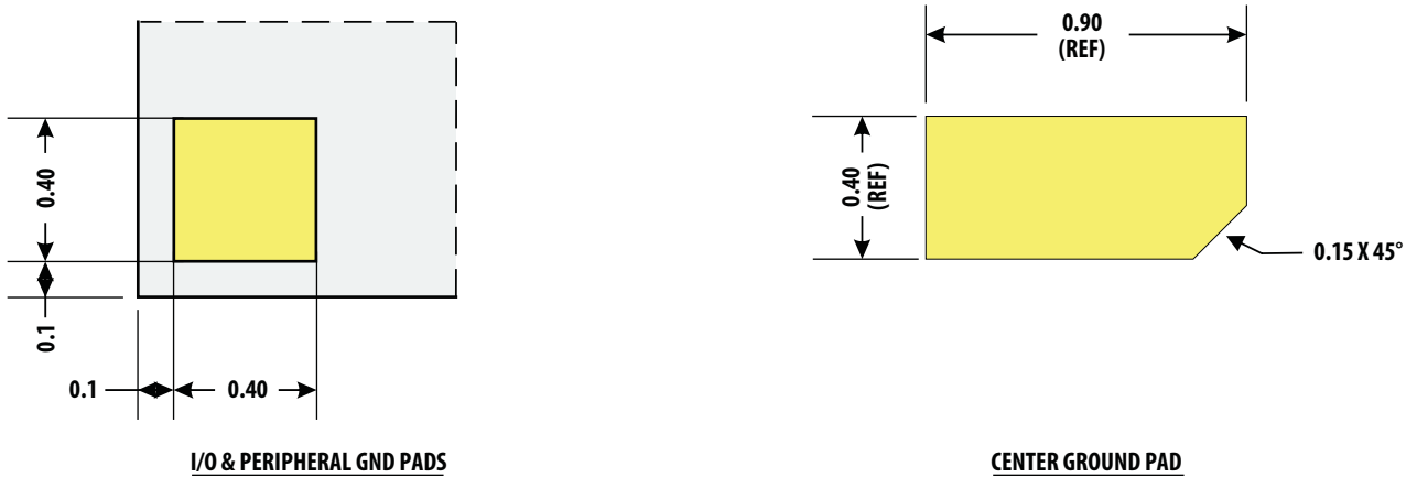
Figure 21. Pad Detail
