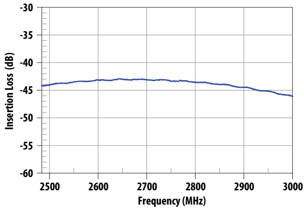
Figure 15. Ant-Rx Rejection, 2484 –3000 MHz
