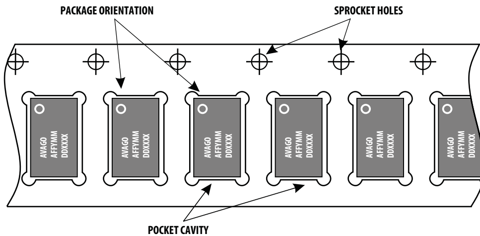
Figure 31. Unit Orientation in SMT Tape
