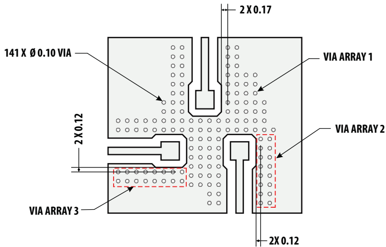
Figure 23. PCB Layout, Via Detail
