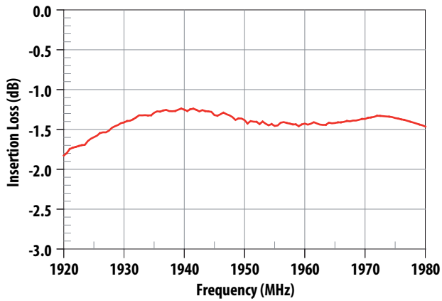
Figure 1. Tx-Ant Insertion Loss
