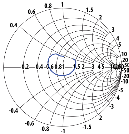
Figure 17. Rx Port Impedance in Rx Band
