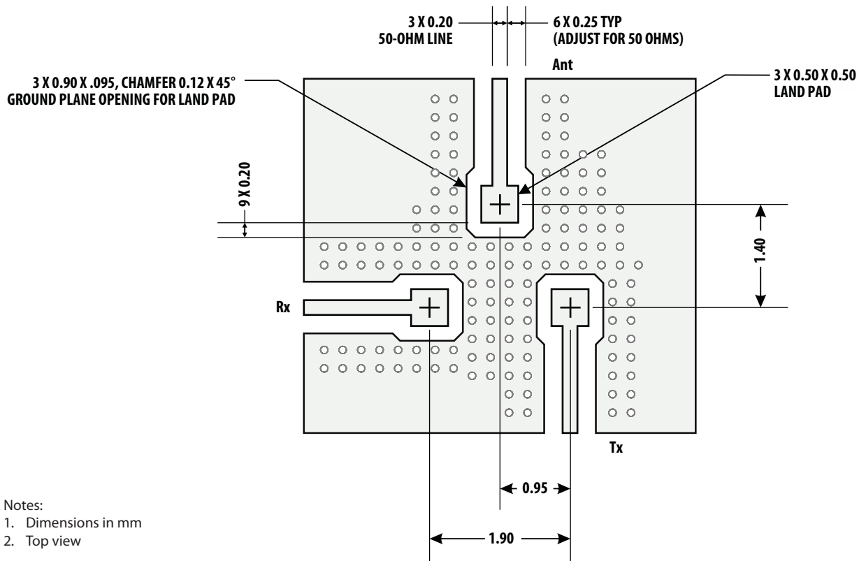
Figure 22. Suggested PCB Layout
