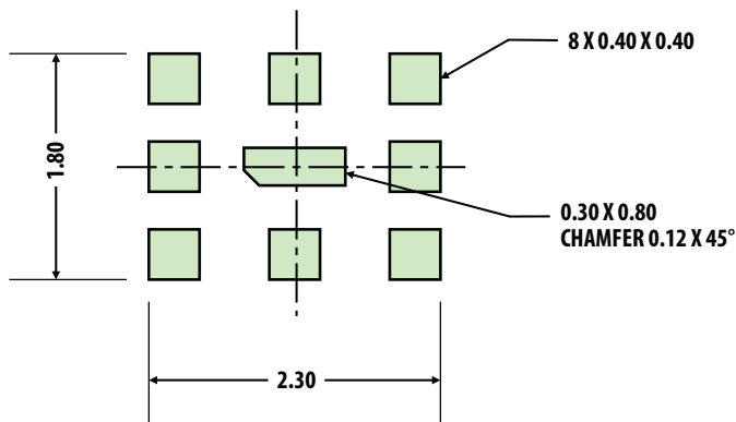
Figure 24. ACMD-7614 Foot Print Superposed on PCB Layout
