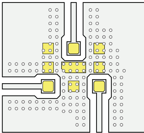
Figure 24. ACMD-7614 Foot Print Superposed on PCB Layout
