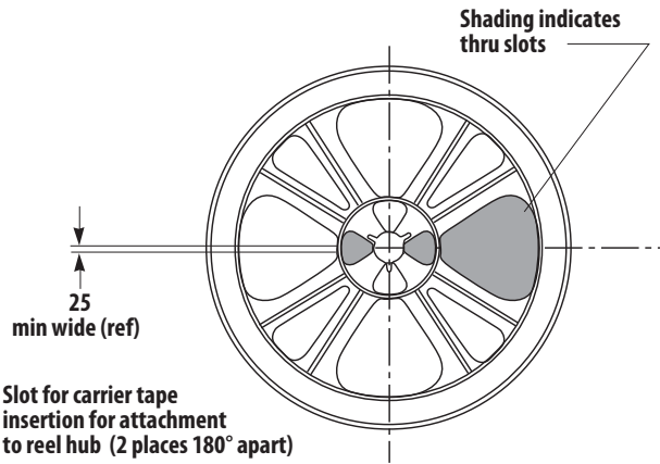
Figure 32. SMT Reel Drawing
