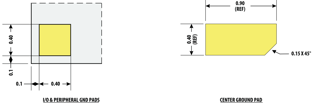
Figure 24. Pad Detail
