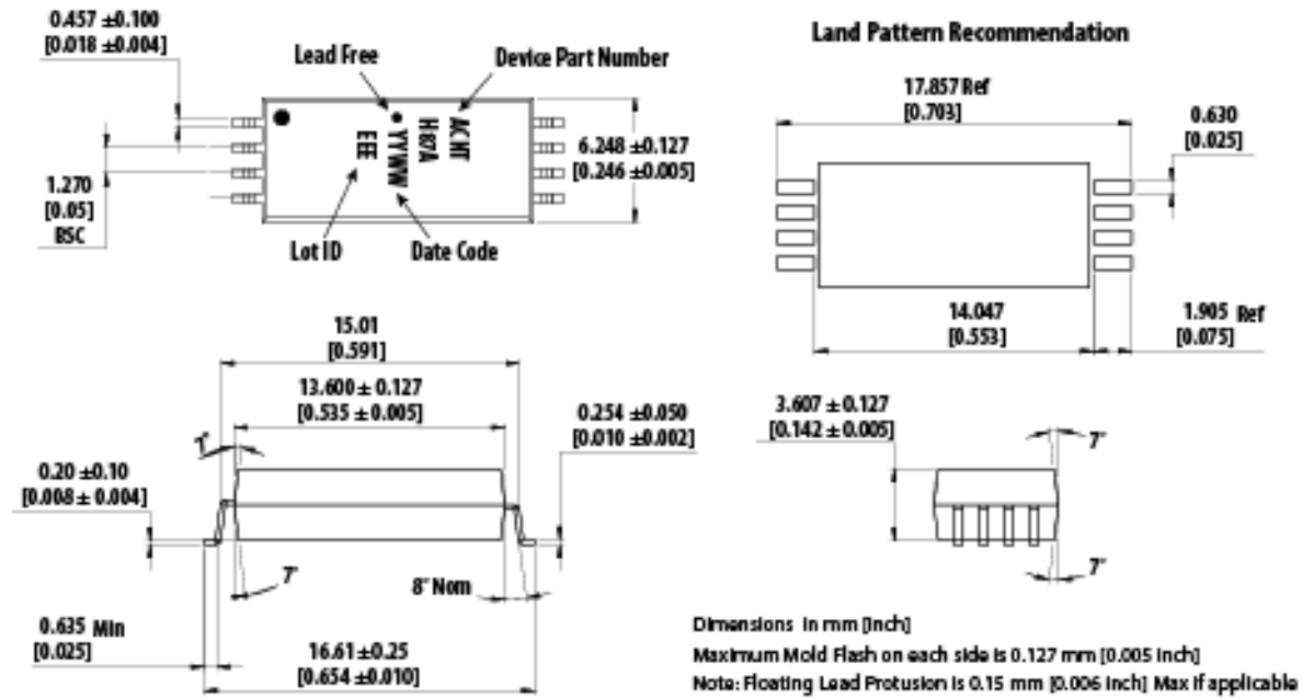
Figure 2 15-mm Stretched SO-8 Package
