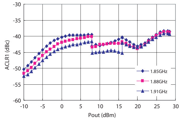
Figure 4. Adjacent Channel Leakage Ratio 1 vs. Output Power
