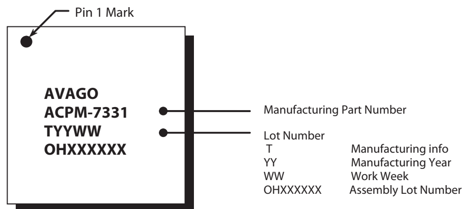
Figure 14. Marking Specifications
