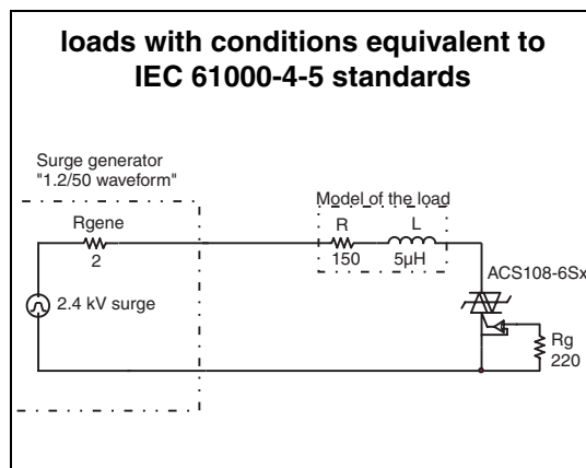
Figure 19. Overvoltage ruggedness test circuit for resistive and inductive
