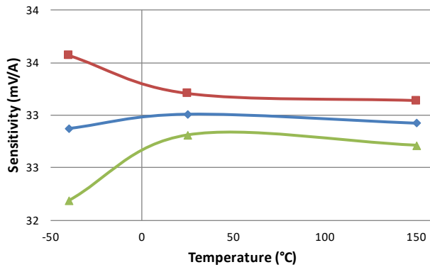
Sensitivity vs. Temperature
