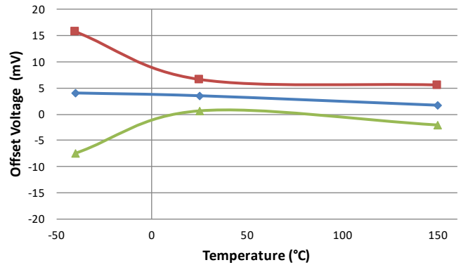
Offset Voltage vs. Temperature
