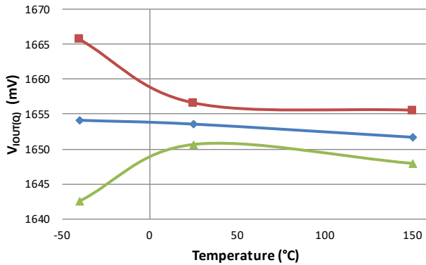
Zero Current Output Voltage vs. Temperature
