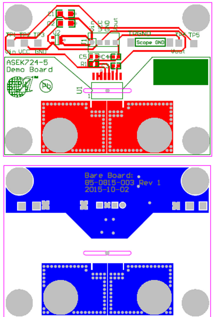
Figure 7: Top and bottom layers for ASEK724/5 MA evaluation board
