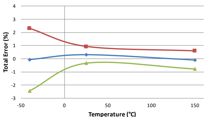
Total Error vs. Temperature
