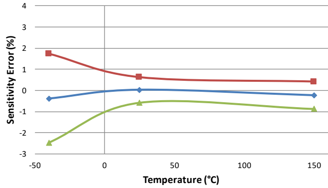
Sensitivity Error vs. Temperature
