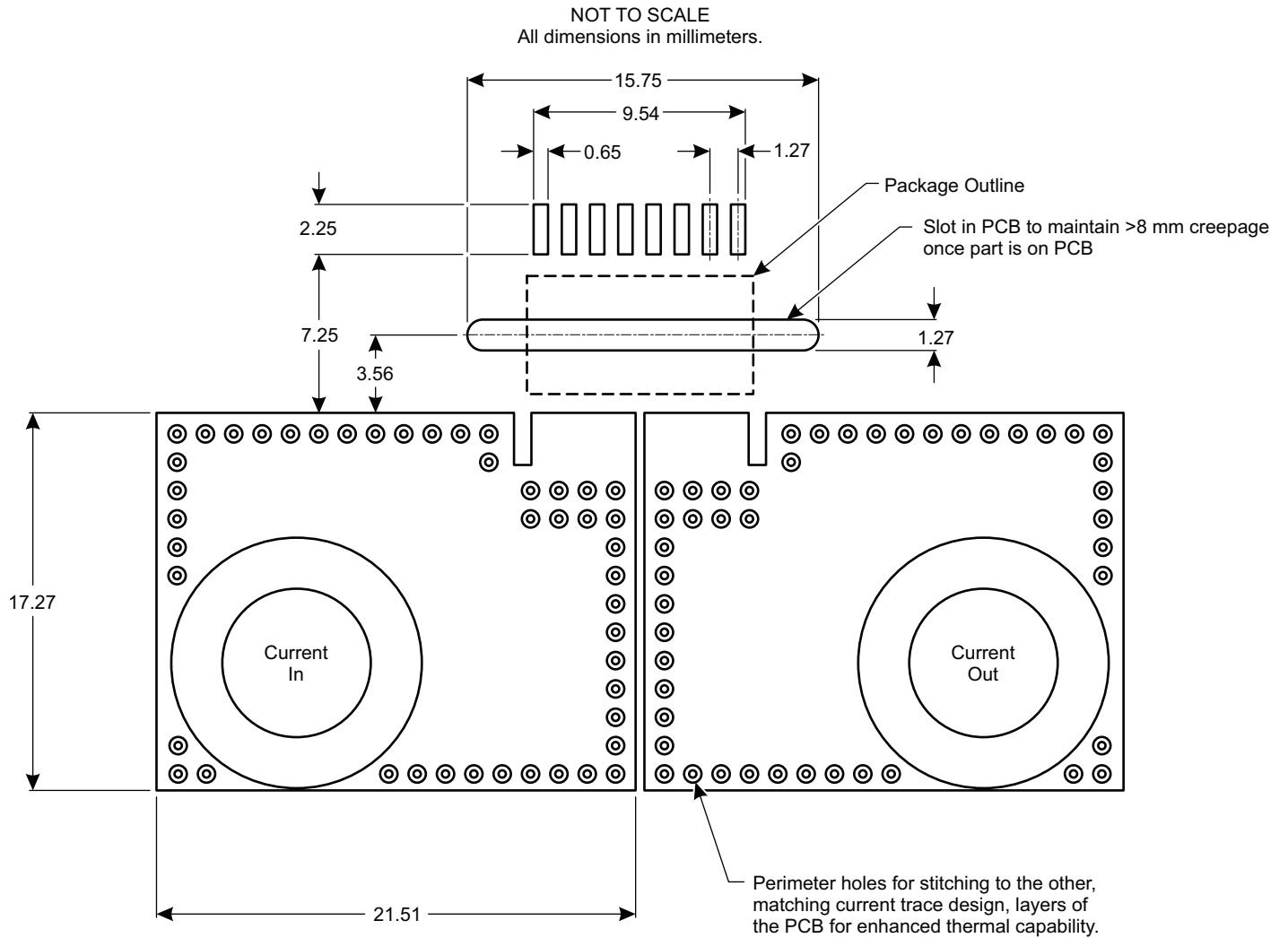
Figure 8: High-Isolation PCB Layout
