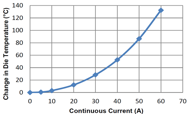
Figure 6: Self-heating in the MA package due to current flow
