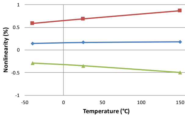
Nonlinearity vs. Temperature
