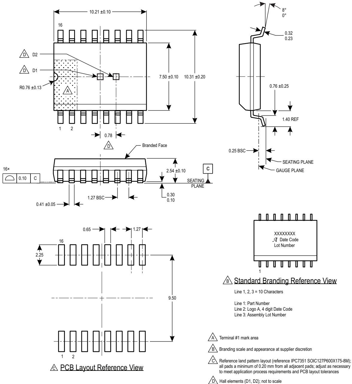
Figure 9: Package MA, 16-Pin SOICW
