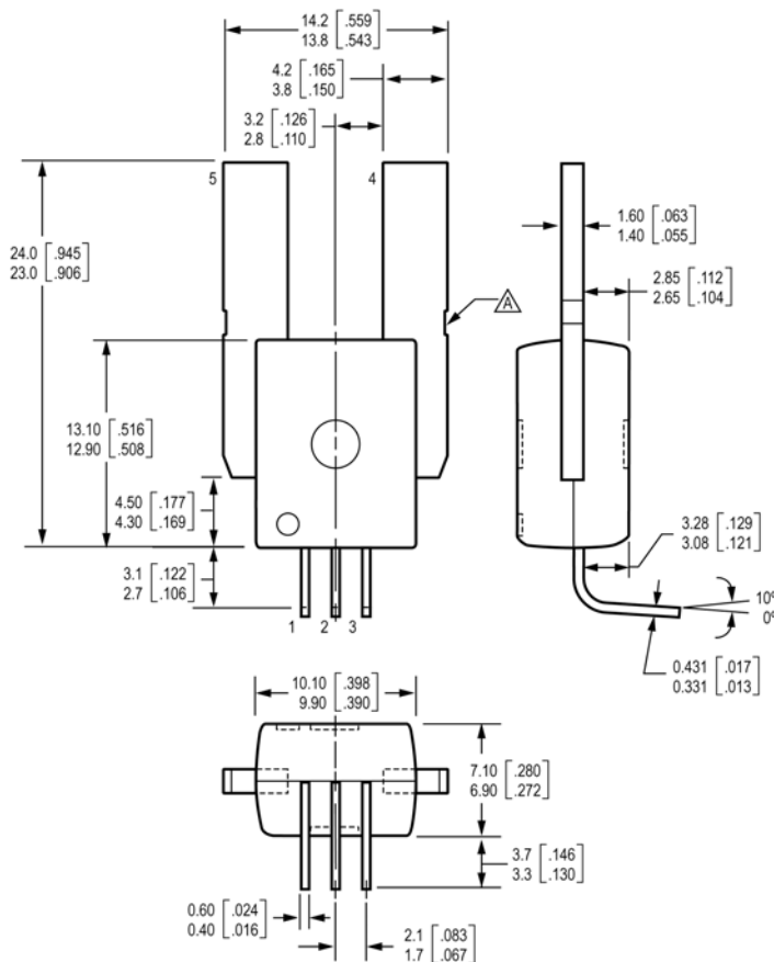
Package CB-PSF
