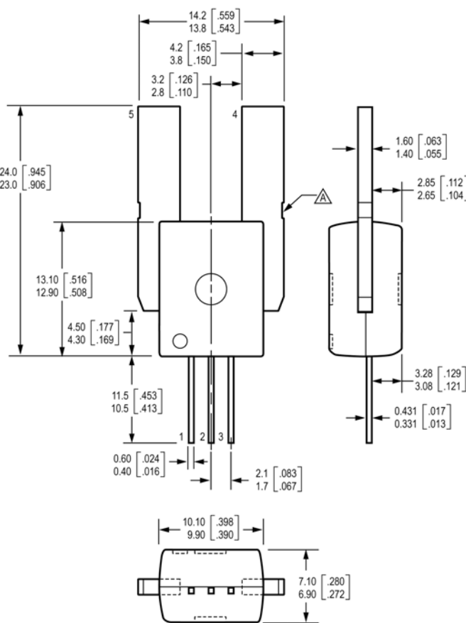
Package CB-PSS
