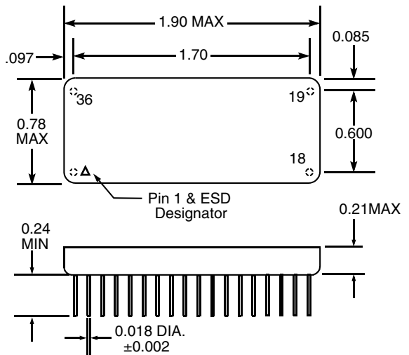
Plug In Package Outline
