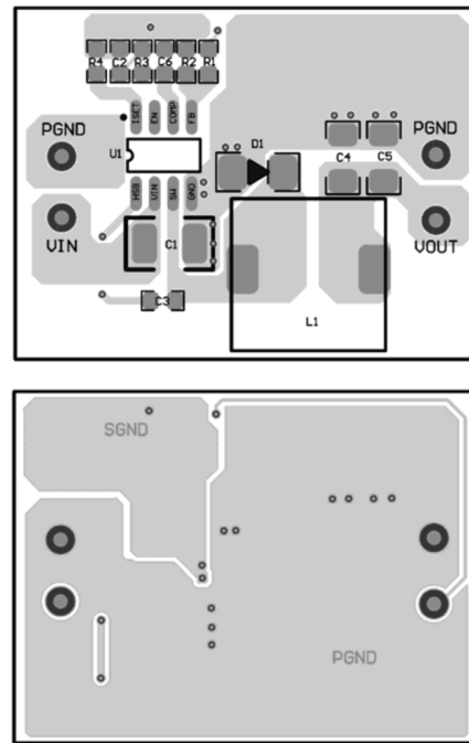
Figure 8: PCB Layout
