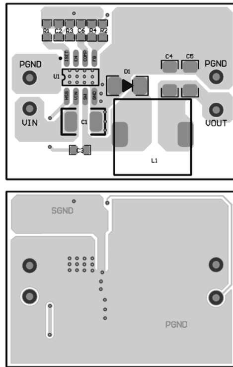
Figure 8: PCB Layout
