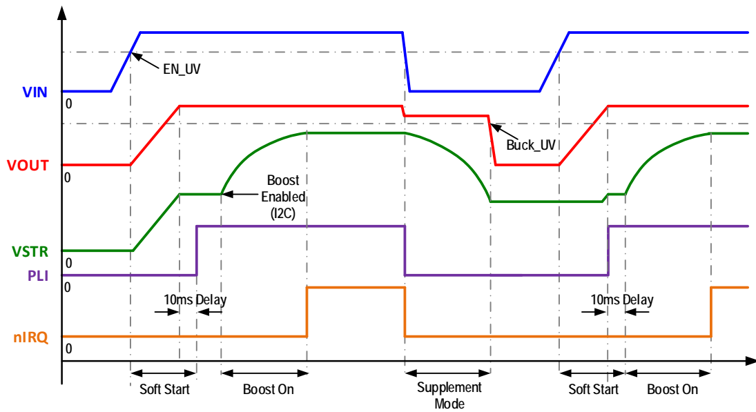
Figure 4: Operation states
