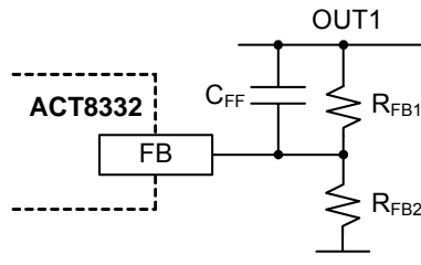
Figure 4: Output Voltage Programming
