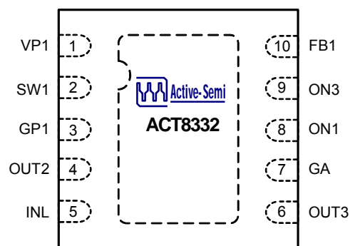
Thin - DFN (TDFN 33-10)
