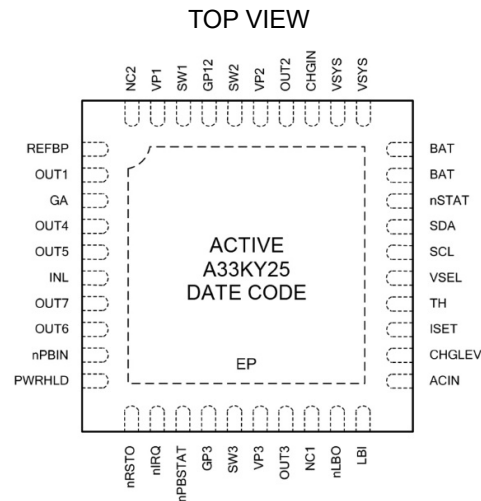
Thin - QFN (TQFN55-40)
