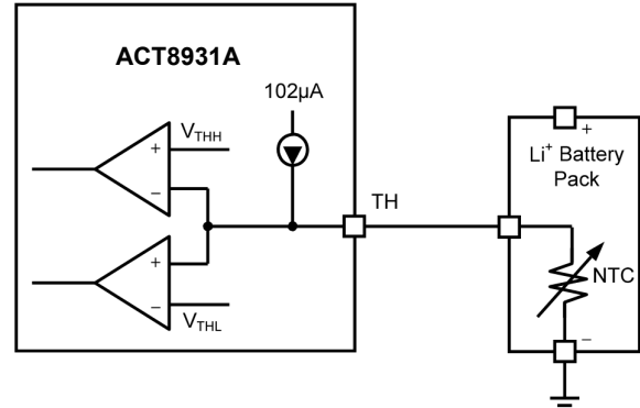
Figure 6 : Simple Configuration
