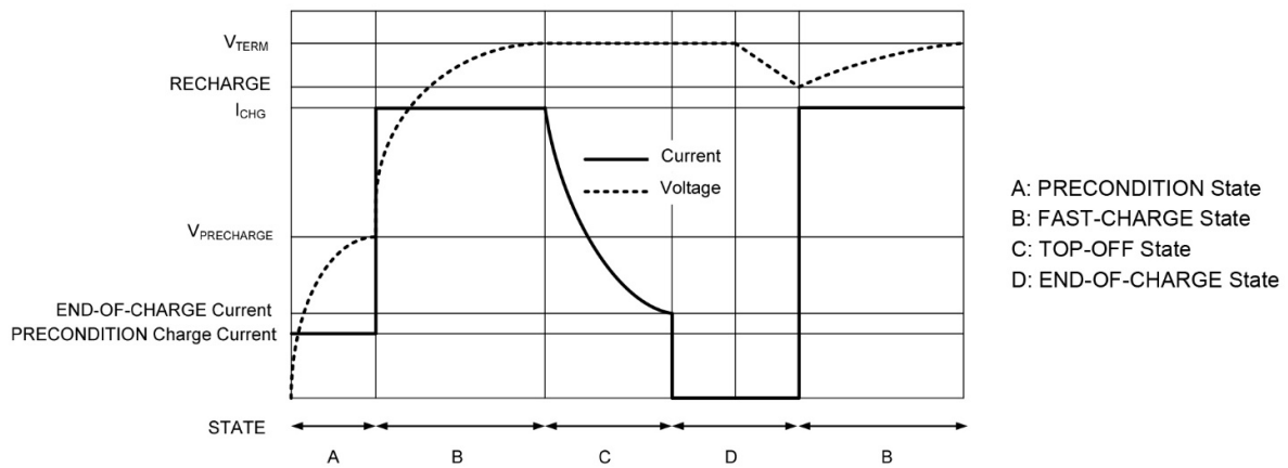
Figure 4 : Typical Li+ charge profile and ACT8931A charge states
