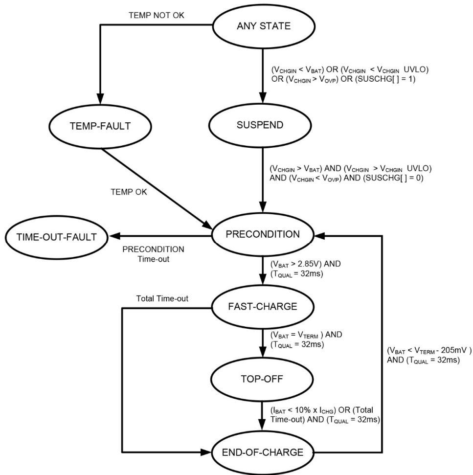
Figure 5 : Charger State Diagram
