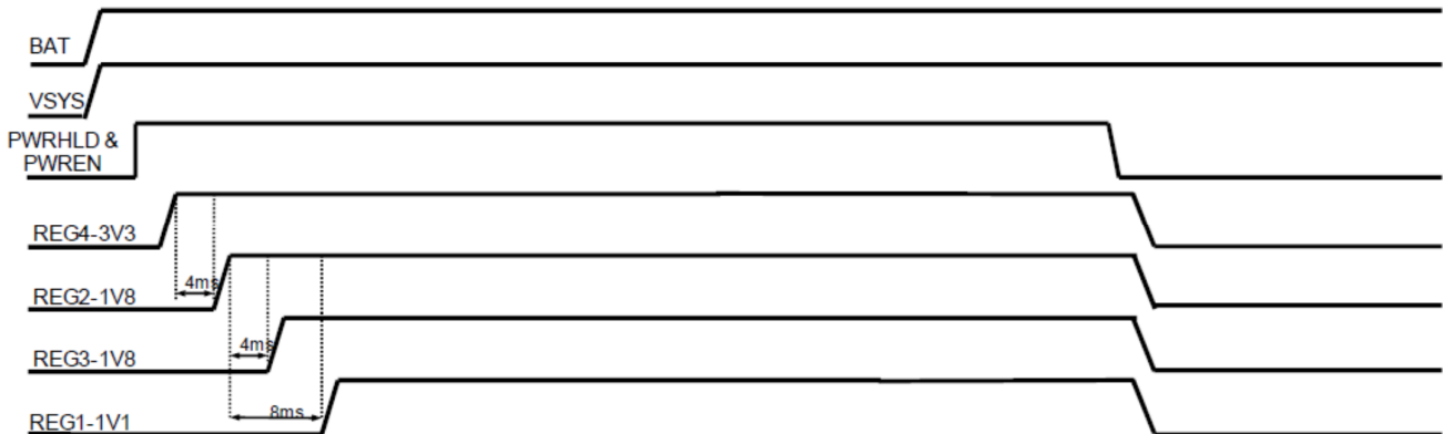
Figure 2: ACT8946AQJ203-T Enable/Disable Sequence
