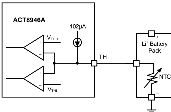
Figure 3: Simple Configuration
