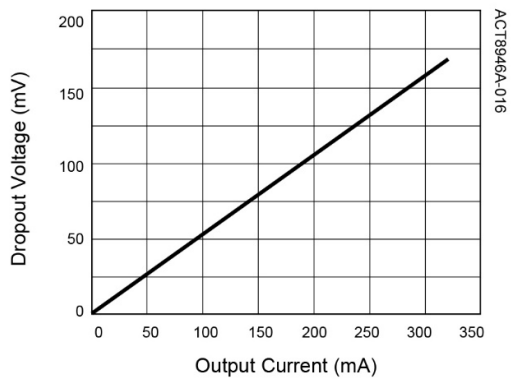
REG4, 6 Dropout Voltage vs. Output Current
