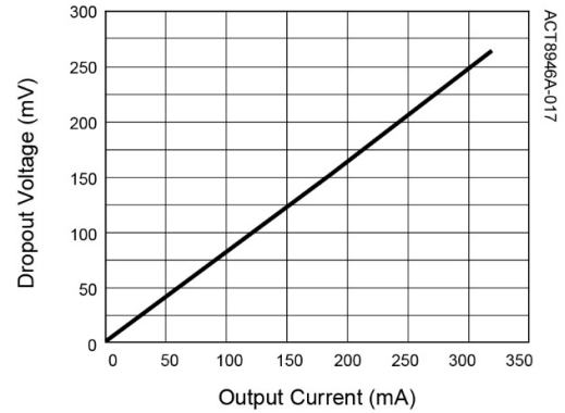
REG5, 7 Dropout Voltage vs. Output Current
