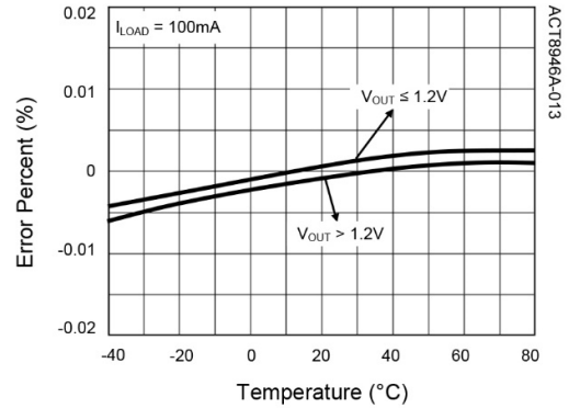
REG1, 2, 3 Output Voltage vs. Temperature
