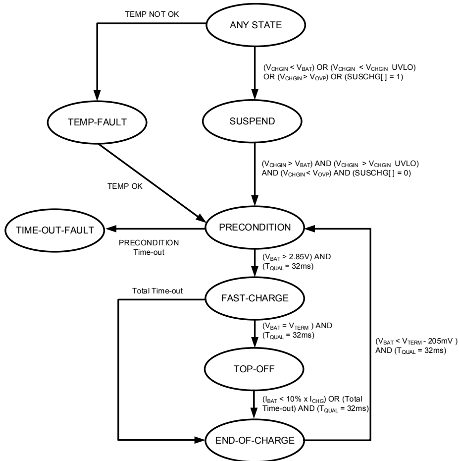
Figure 5: Charger State Diagram
