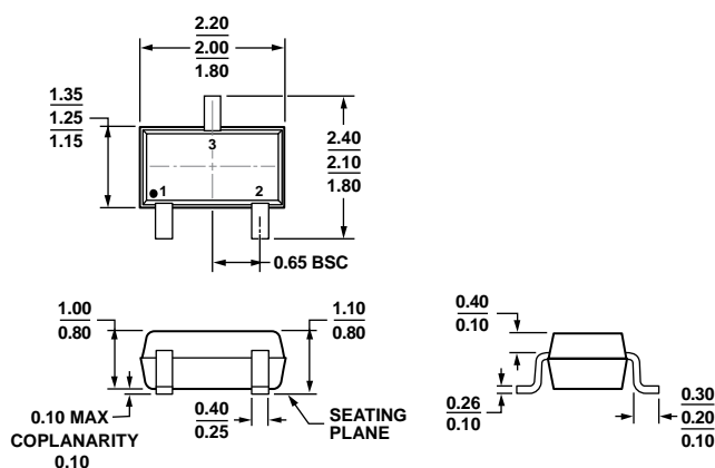
Figure 28. 3-Lead Thin Shrink Small Outline Transistor Package [SC70] (KS-3)
