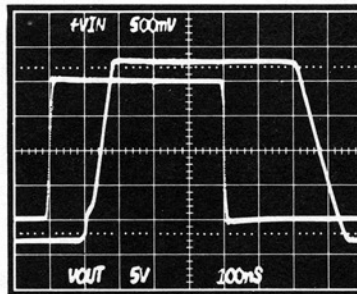
Figure 24b. Overdrive Recovery Response
