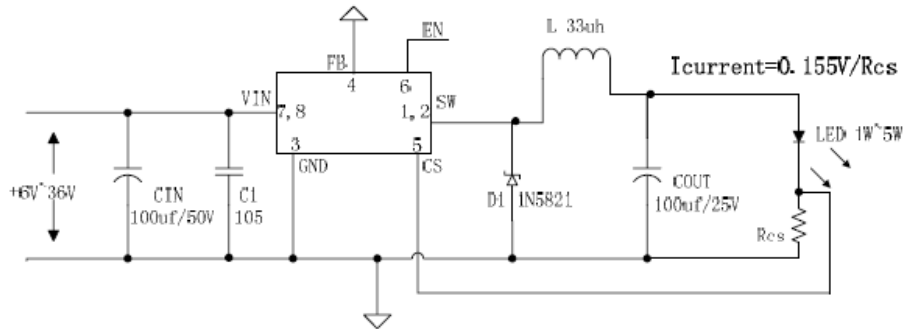
Figure5. AD4021 Typical Application Circuit (LED Constant Current Driver)
