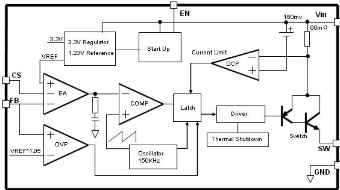
Figure3. Function Block Diagram of AD4021
