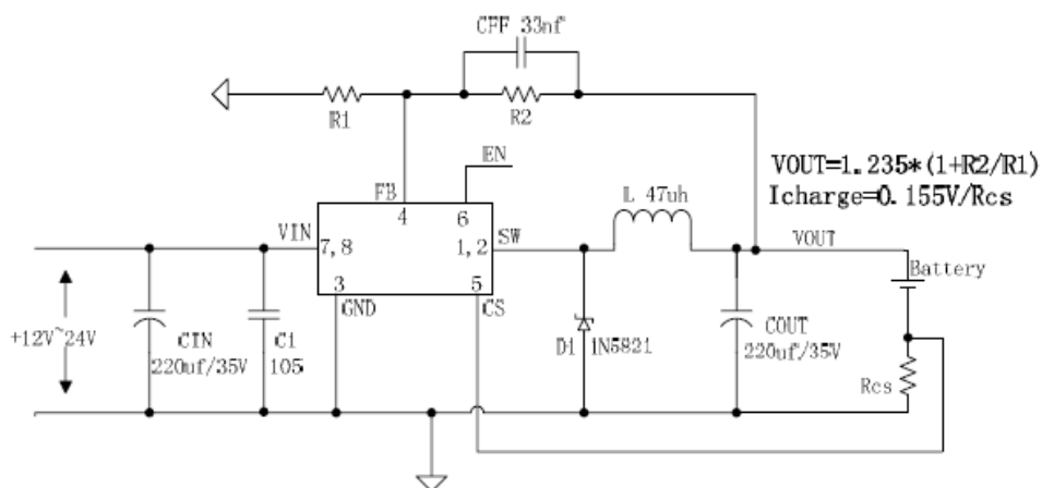
Figure4. AD4021 Typical Application Circuit (Li Battery Charger)
