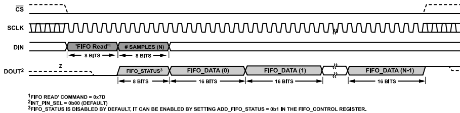
Figure 106. FIFO Readback (FIFO_STATUS Append On and FIFO_HEADER Append Off)
