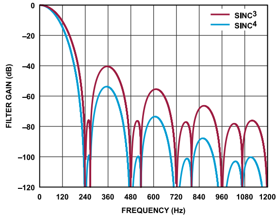
Figure 86. Sinc 3 and Sinc 4 Filter Response (FS = 0d10)
