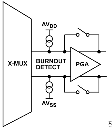
Figure 102. Burnout Currents
