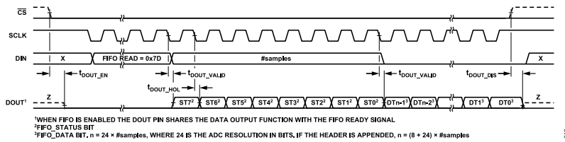
Figure 12. FIFO Readback Timing Diagram
