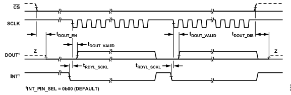
Figure 10. Continuous Read Mode Timing
