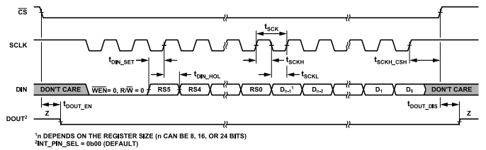
Figure 5. Write Cycle Timing Diagram, 3-Wire Mode (CSB_EN Bit Set to 0), CS Pin Used to Tristate the DOUT Pin
