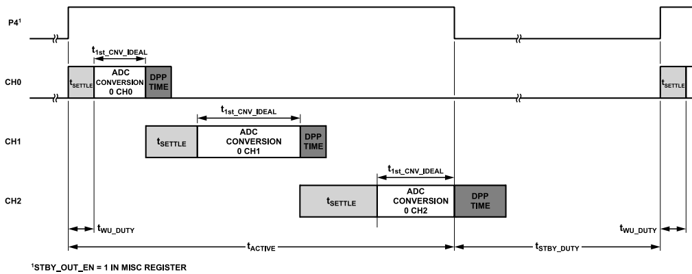
Figure 96. Example of Autonomous Duty Cycling Mode
