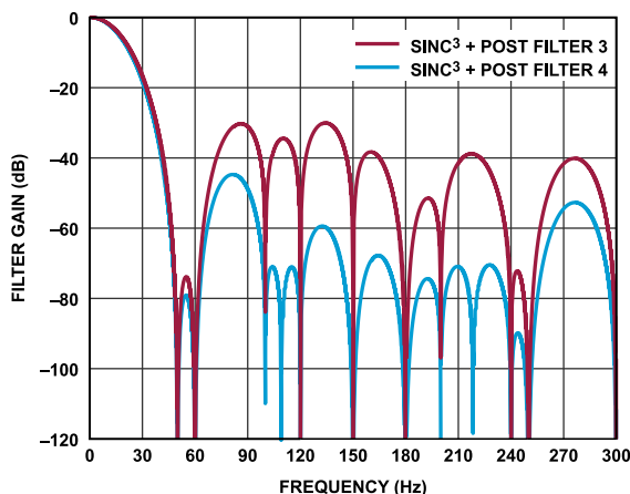
Figure 88. Post Filter 3 and Post Filter 4 Response
