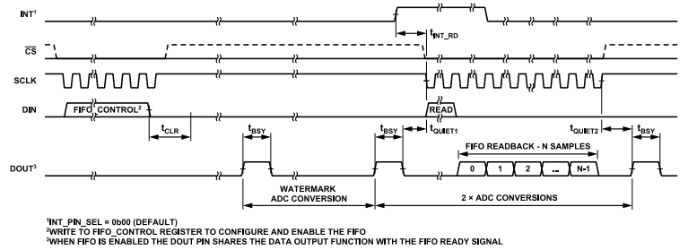
Figure 11. FIFO Timing with Watermark Interrupt
