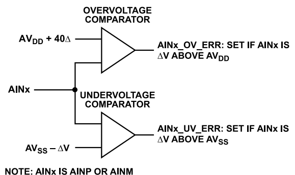
Figure 99. Analog Input Overvoltage/Undervoltage Monitors
