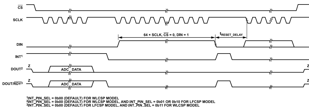
Figure 76. Software Reset Timing Diagram
