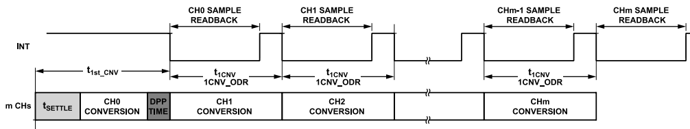
Figure 94. Example of Standard Sequencing Through Multiple Channels with Same Configuration and No Repeat Conversion
