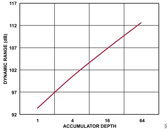
Figure 18. Dynamic Range vs. Accumulator Depth
