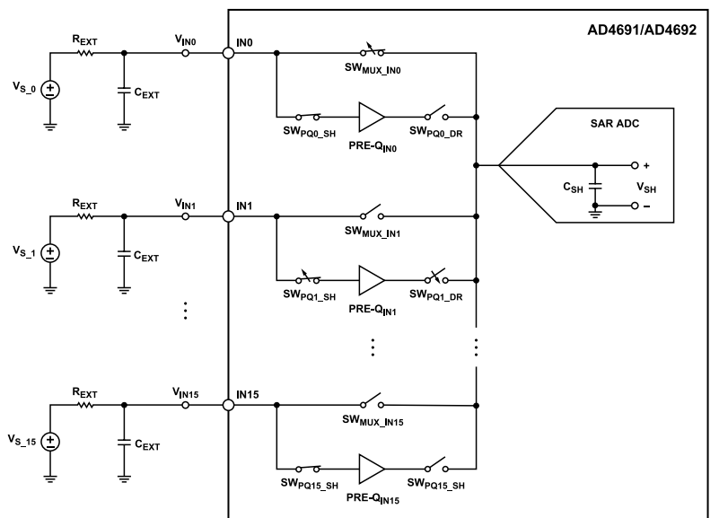
Figure 51. Precharge Buffer Simplified Circuit Diagram
