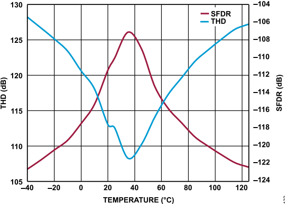
Figure 17. THD and SFDR vs. Temperature
