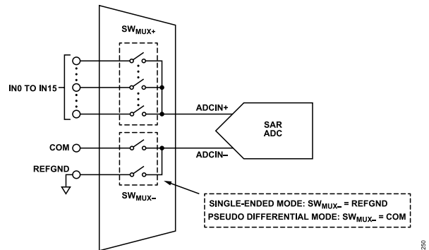
Figure 50. Multiplexer Simplified Connection Diagram
