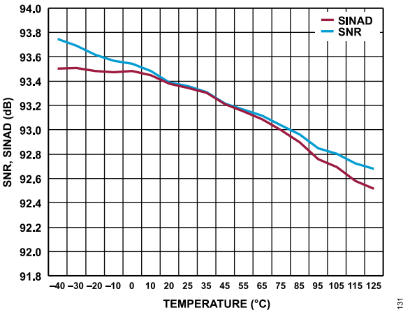
Figure 14. SNR and SINAD vs. Temperature
