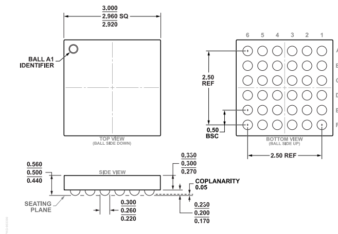
Figure 103. 36-Ball Wafer Level Chip Scale Package (WLCSP) (CB-36-5)
