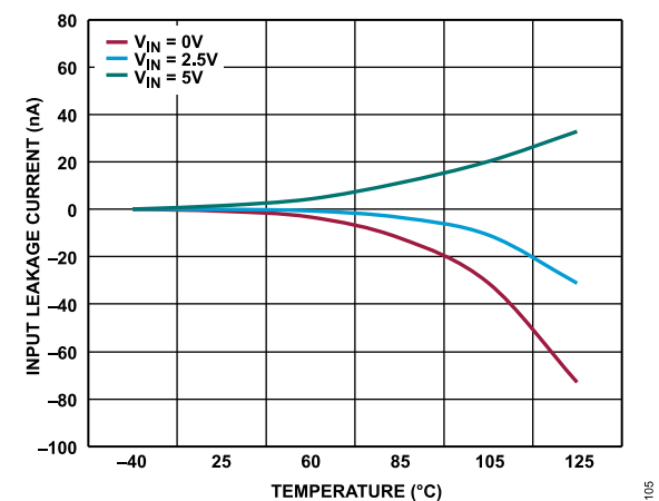
Figure 29. Analog Input Leakage Current vs. Temperature
