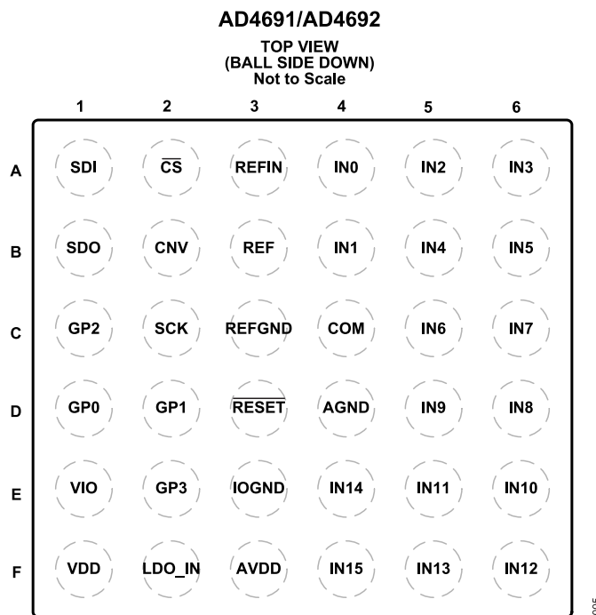
Figure 5. AD4691/AD4692 WLCSP Pin Configuration
