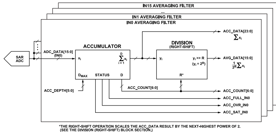
Figure 60. Averaging Filter Simplified Diagram
