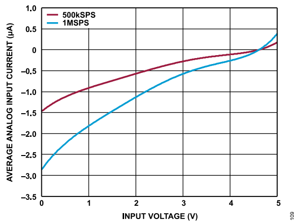
Figure 27. Average Analog Input Current vs. Input Voltage, f_s = 1\text{MSPS} and 500\text{kSPS}
