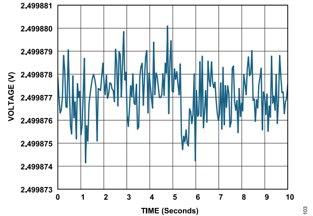
Figure 21. 1/f Noise (0.1Hz to 10Hz Bandwidth), 50kSPS
