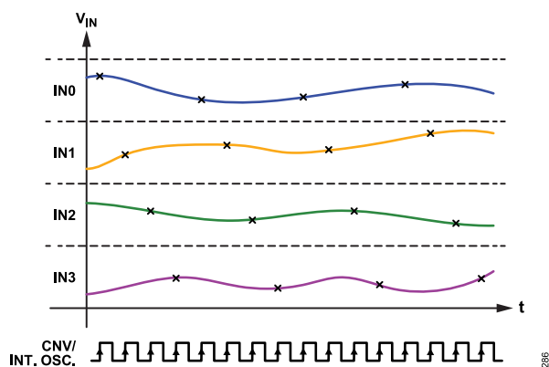
Figure 86. Interleaved Sequencing with AD4691/AD4692 (Averaging by 4)
