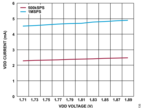
Figure 37. VDD Current vs. VDD Voltage
