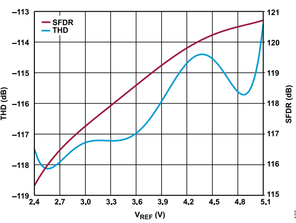
Figure 16. THD and SFDR vs. V_{REF}
