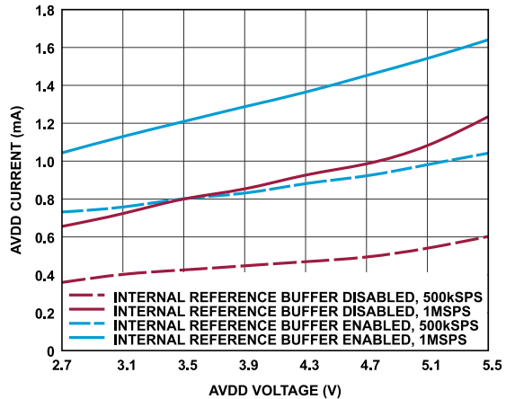
Figure 31. AVDD Current vs. AVDD Voltage
