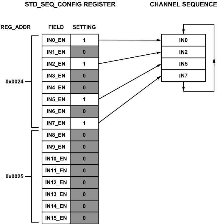
Figure 56. Standard Sequencer Simplified Diagram
