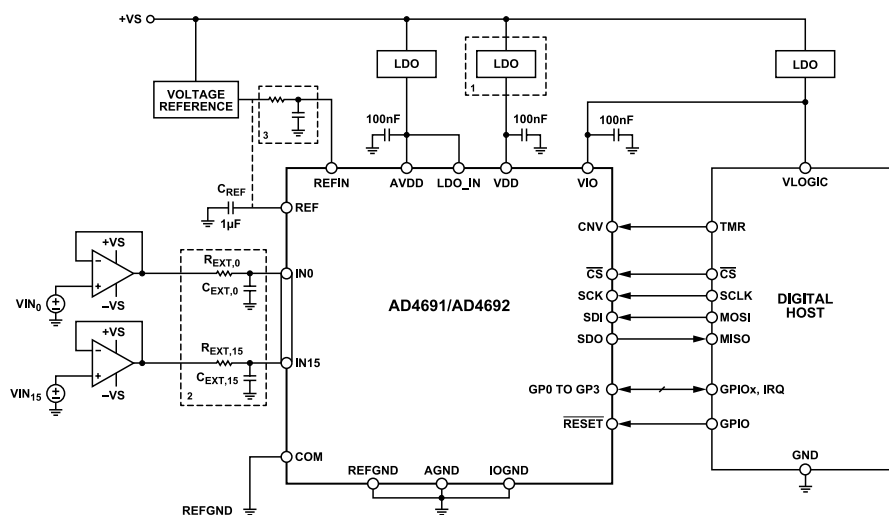
Figure 84. AD4691/AD4692 Typical Connection Diagram
