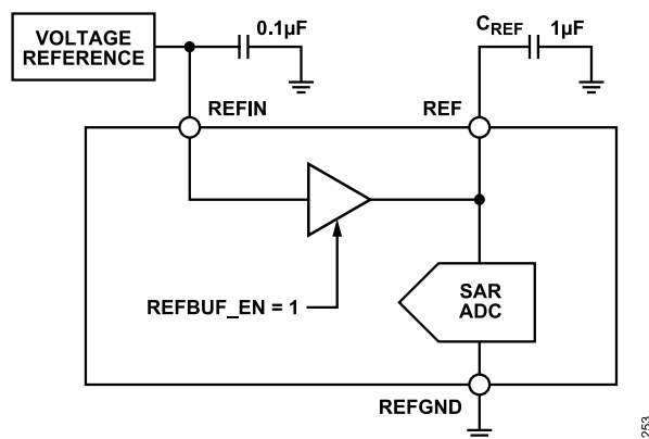
Figure 53. Internal Reference Buffer Simplified Schematic
