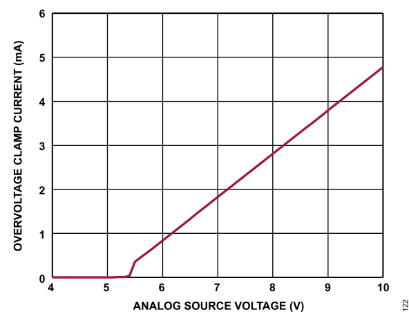
Figure 28. Overvoltage Protection Clamp Current vs. Analog Source Voltage
