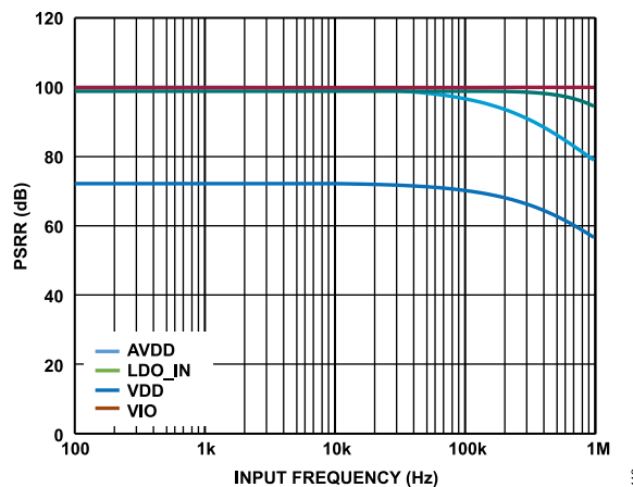
Figure 20. Power Supply Rejection Ratio (PSRR) vs. Input Frequency
