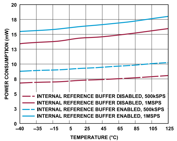
Figure 43. Power Consumption vs. Temperature (Internal LDO Disabled)
