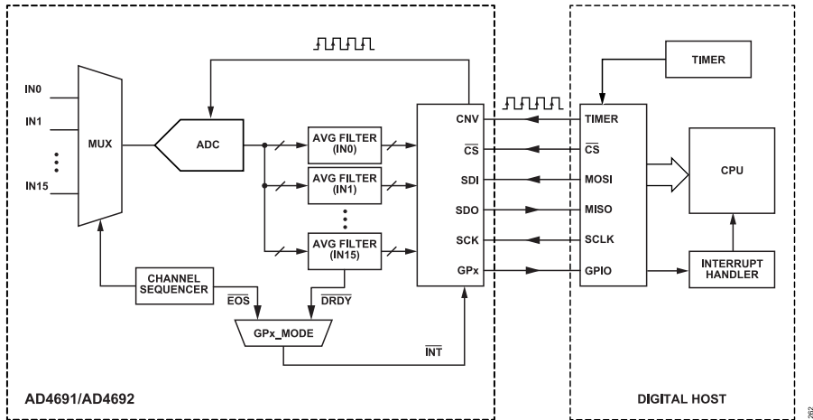
Figure 62. CNV Clock Mode Example Connection Diagram
