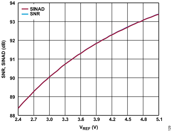
Figure 13. SNR and SINAD vs. V_{REF}
