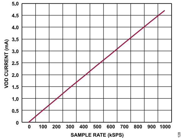
Figure 36. VDD Current vs. Sample Rate
