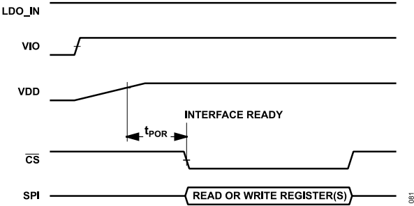
Figure 81. VIO POR Timing Diagram (VDD Supplied Internally)
