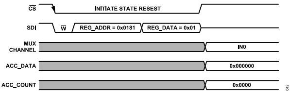
Figure 83. State Reset Timing Diagram
