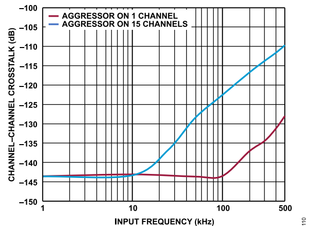
Figure 23. Channel-to-Channel Crosstalk vs. Input Frequency
