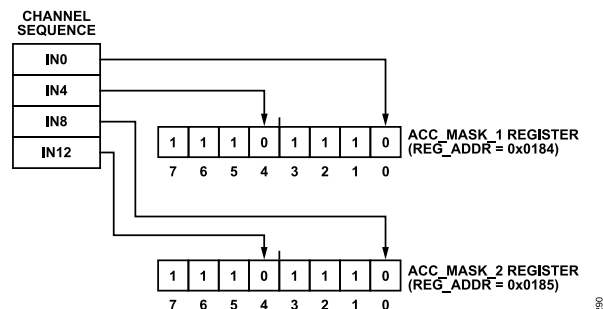
Figure 90. Mask Bit Setting vs. Channel Sequence Example
