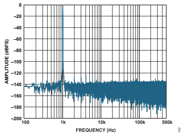
Figure 22. Fast Fourier Transform (FFT), f_{IN} = 1\text{kHz} , V_{REF} = 5\text{V}
