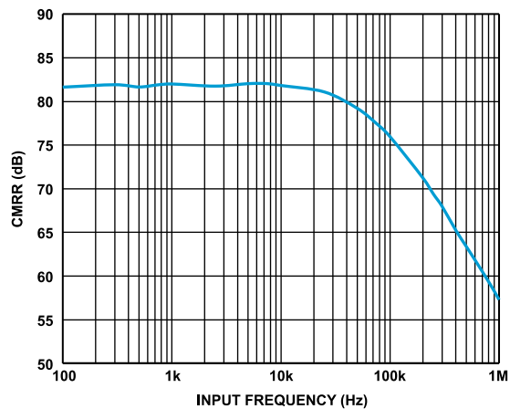
Figure 19. CMRR vs. Input Frequency
