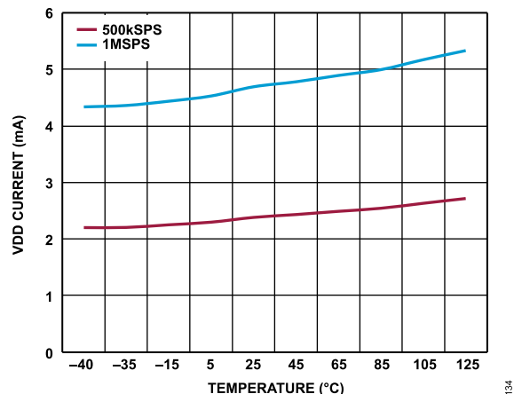
Figure 38. VDD Current vs. Temperature
