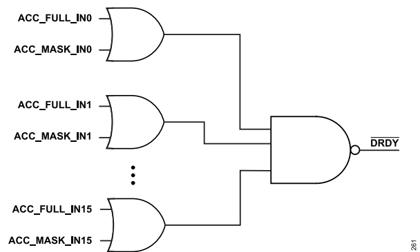
Figure 61. \overline{\text{DRDY}} Masking Logic Diagram (Simplified)
