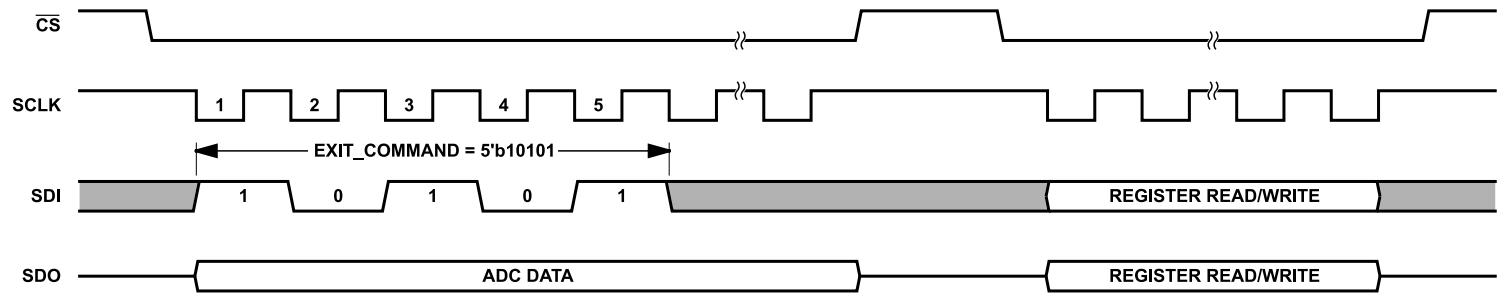
Figure 73. Exit Command Timing Diagram
