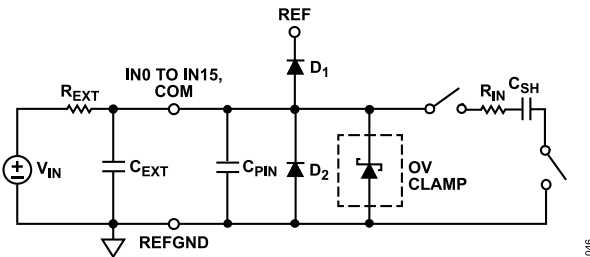
Figure 49. Equivalent Analog Input Circuit
