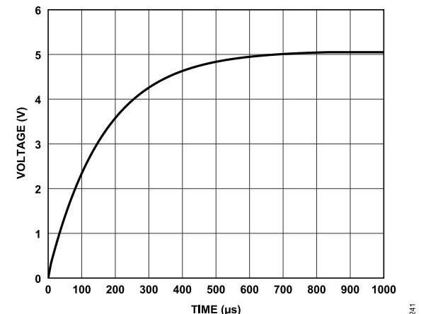
Figure 41. V_{REF} vs. Time (Internal Reference Buffer Enabled), C_{REF} = 1\mu F
