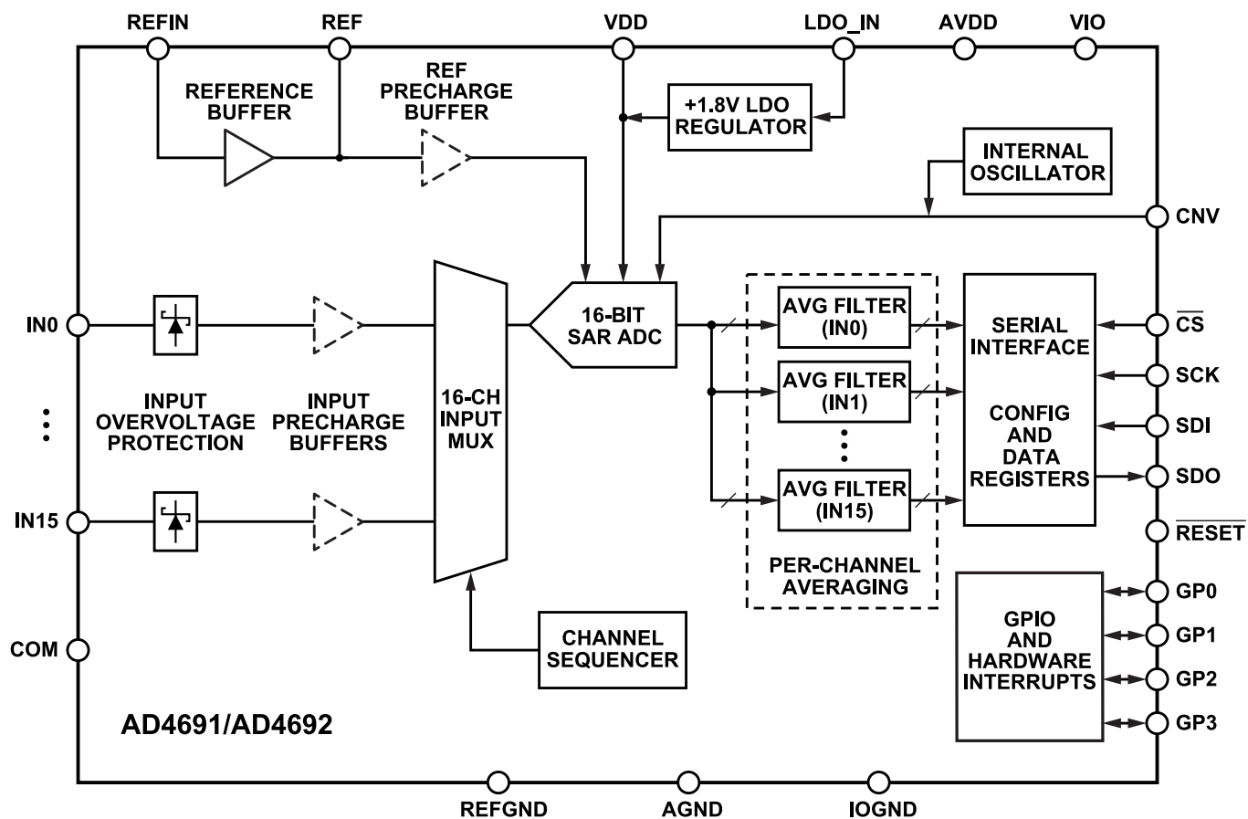
Figure 1. AD4691/AD4692 Functional Block Diagram
