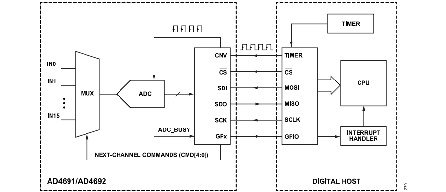
Figure 70. Manual Mode Example Connection Diagram
