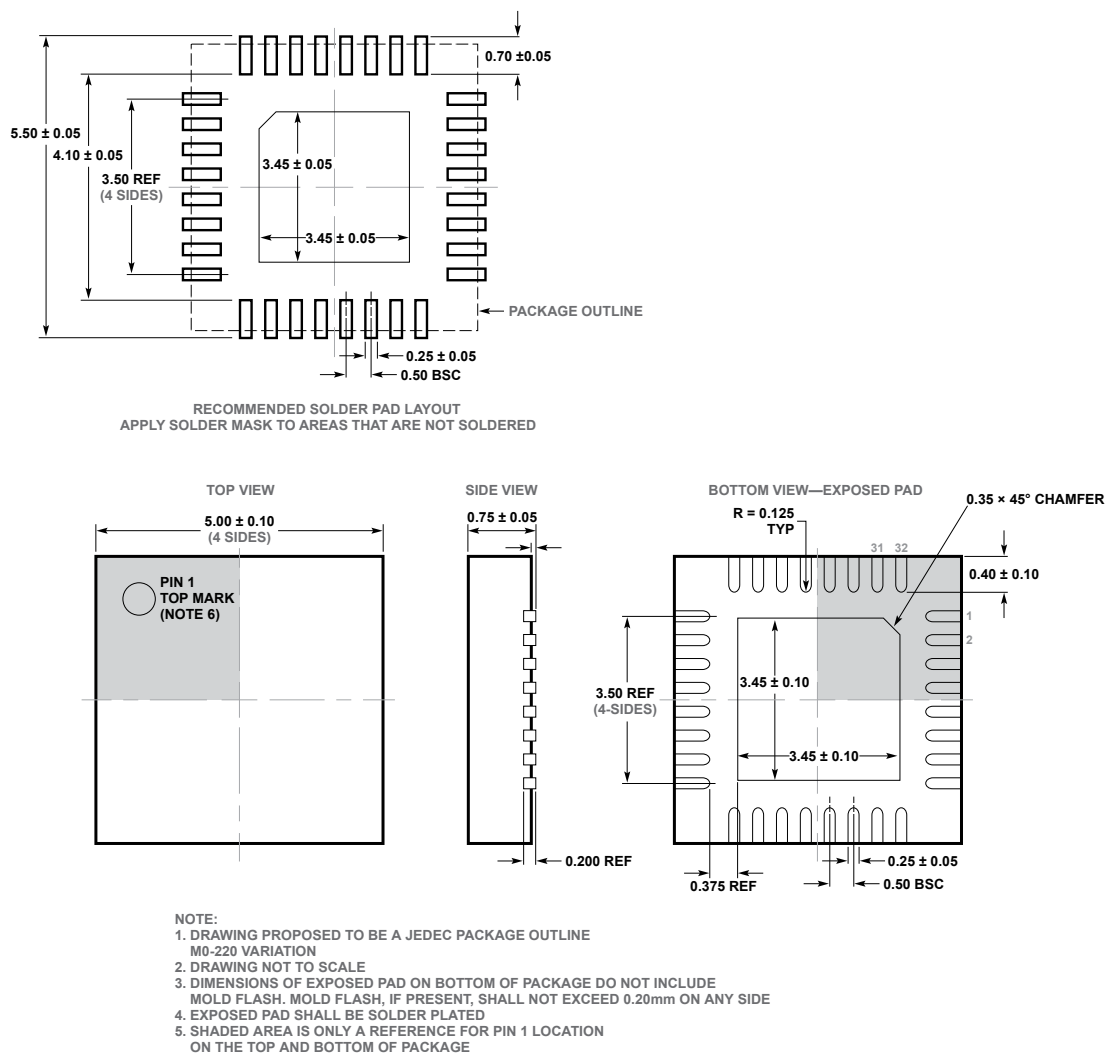
Figure 102. 32-Lead Lead Frame Chip Scale Package [LFCSP] 5mm × 5mm Body and 0.75mm Package Height (CP-32-39) Dimensions shown in millimeters
