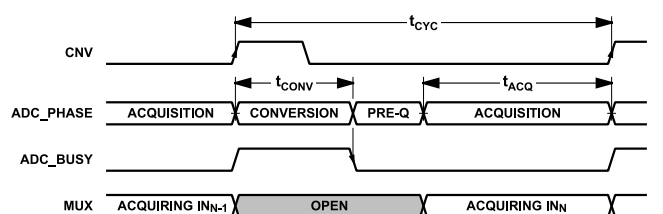
Figure 47. ADC Phase Timing Diagram
