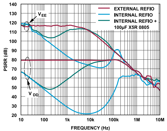
Figure 32. PSRR vs. Frequency, Internal and External Reference
