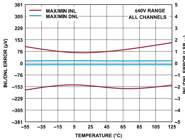
Figure 44. INL/DNL Error vs. Temperature
