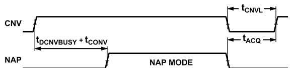
Figure 62. Nap Mode Timing for the AD4856
