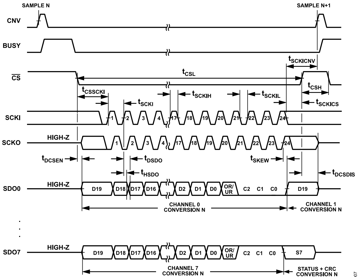
Figure 6. CMOS Conversion Data Bus Timing
