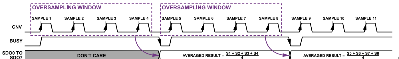
Figure 51. Oversampling Mode with 4× Oversampling Ratio (OS_RATIO = 0x1)
