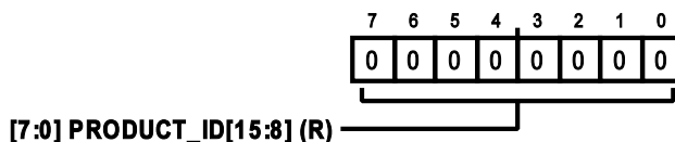
Figure 80. Address: 0x05, Reset: 0x00, Name: PRODUCT_ID_H
