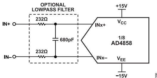
Figure 55. Example Differential Input Filter
