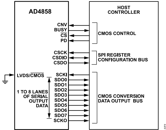
Figure 65. CMOS Conversion Data Output Mode
