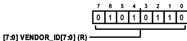
Figure 84. Address: 0x0C, Reset: 0x56, Name: VENDOR_ID_L
