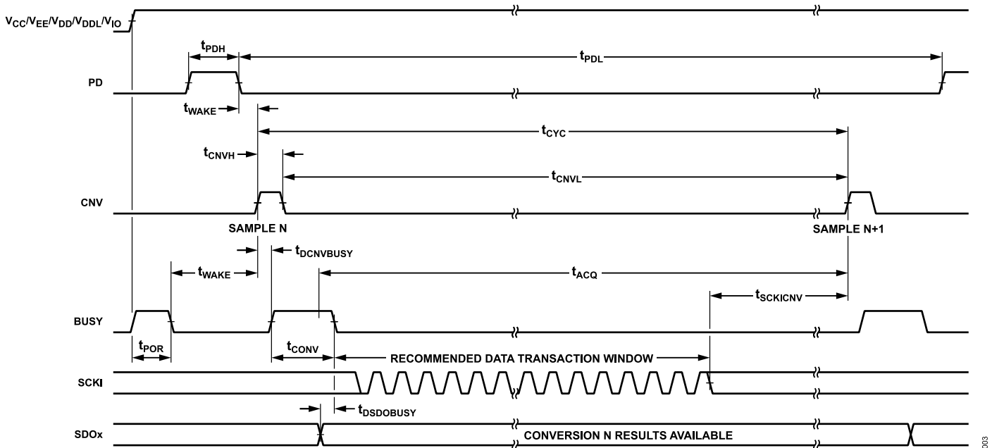
Figure 2. Universal Timing
