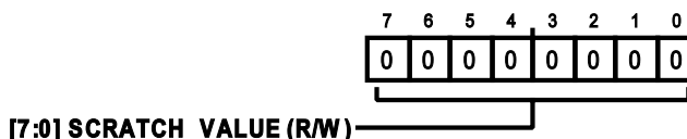
Figure 82. Address: 0x0A, Reset: 0x00, Name: SCRATCH_PAD
