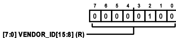
Figure 85. Address: 0x0D, Reset: 0x04, Name: VENDOR_ID_H
