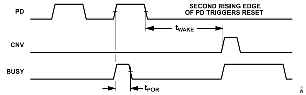
Figure 63. Reset Timing for the AD4858
