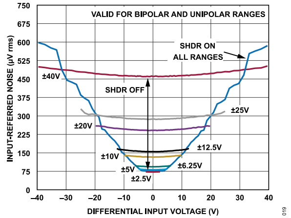
Figure 18. Input-Referred Noise vs. Differential Input Voltage
