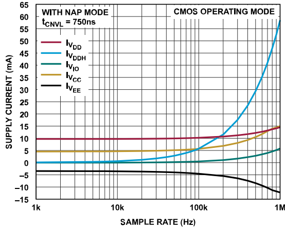
Figure 33. Supply Current vs. Sample Rate
