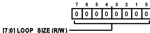
Figure 86. Address: 0x0E, Reset: 0x00, Name: LOOP_CONFIG_A
