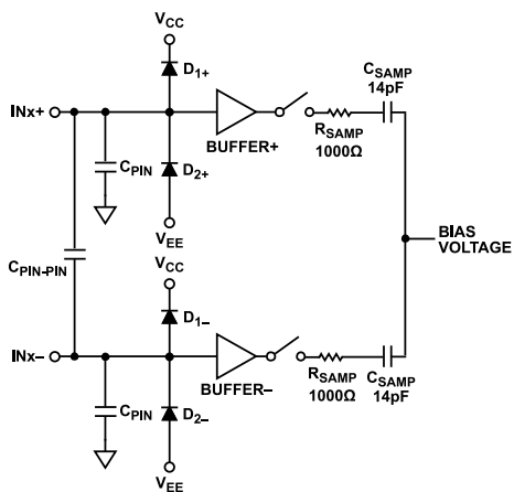
Figure 53. Equivalent Circuit for Differential Analog Inputs, Single Channel
