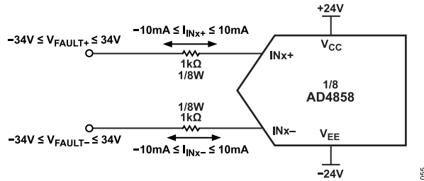
Figure 54. External Series Resistors Limit Latchup Current During Fault Conditions and are Transparent in Normal Operation
