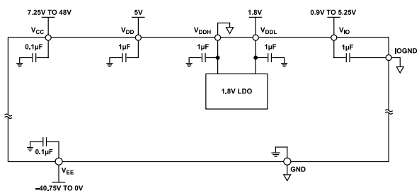
Figure 61. Power Supply Pins of the AD4858 when V_{DDL} is supplied externally
