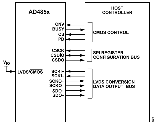
Figure 67. LVDS Conversion Data Output Mode
