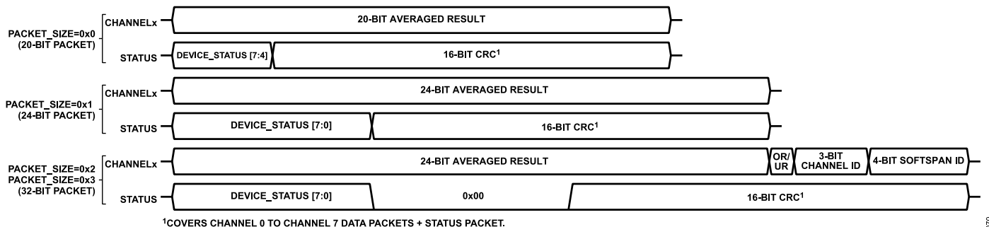
Figure 71. Channel and Status Packet Data Formats in Oversampling Mode (OS_EN = 1), Test Pattern Output is Disabled (TEST_PAT = 0)
