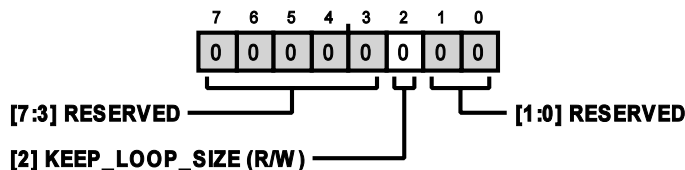
Figure 87. Address: 0x0F, Reset: 0x00, Name: LOOP_CONFIG_B
