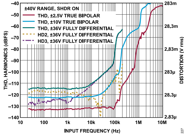
Figure 27. THD, Harmonics vs. Input Frequency
