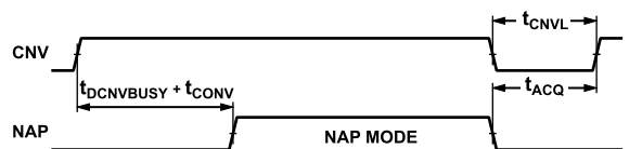
Figure 62. Nap Mode Timing for the AD4858
