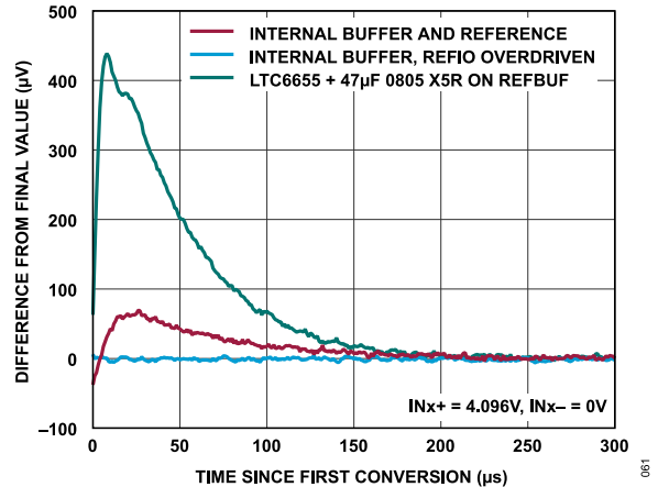
Figure 60. Burst Conversion Response of the AD4858, f_s = 1\text{ MSPS}
