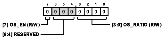
Figure 97. Address: 0x27, Reset: 0x00, Name: OVERSAMPLE
