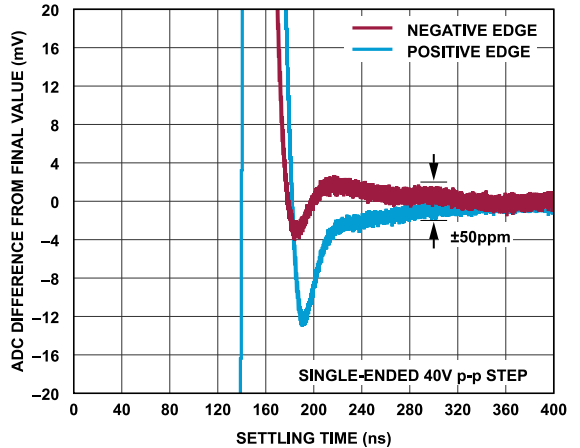
Figure 20. Input Step Response, Fine Settling
