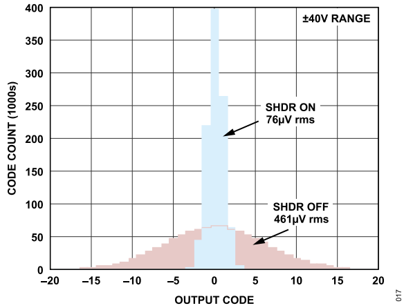
Figure 16. DC Code Histogram, Near Zero Scale
