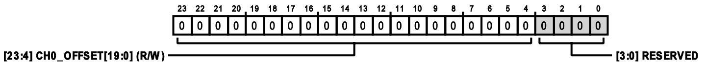
Figure 101. Address: 0x2B to Address: 0x2D, Reset: 0x000000, Name: CH0_OFFSET
