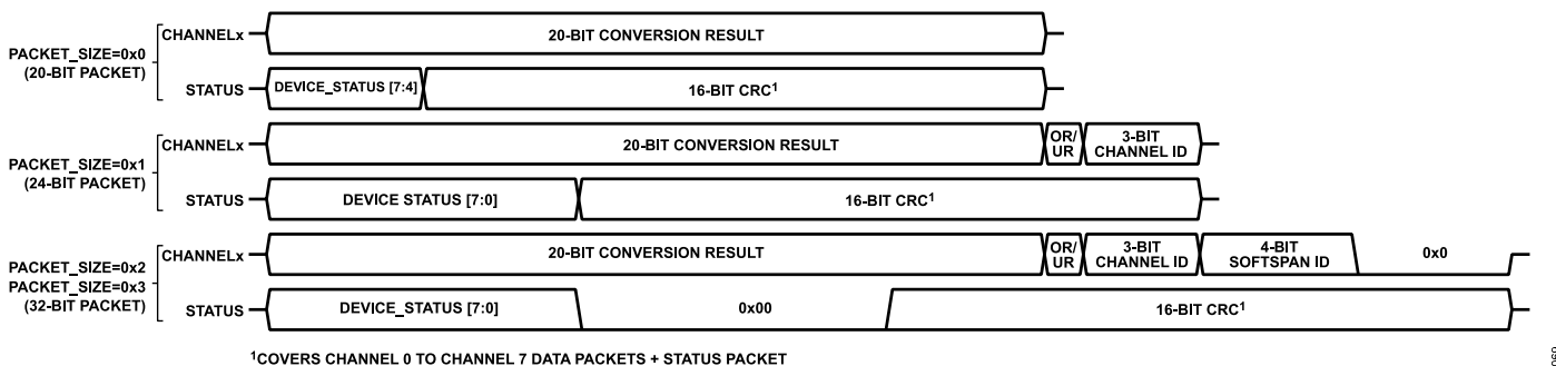
Figure 70. Channel and Status Packet Data Formats in Nonoversampling Mode (OS_EN = 0), Test Pattern Output is Disabled (TEST_PAT = 0)
