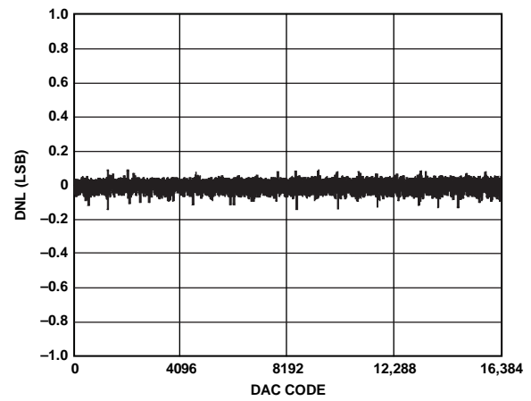
Figure 10. AD5045 DNL
