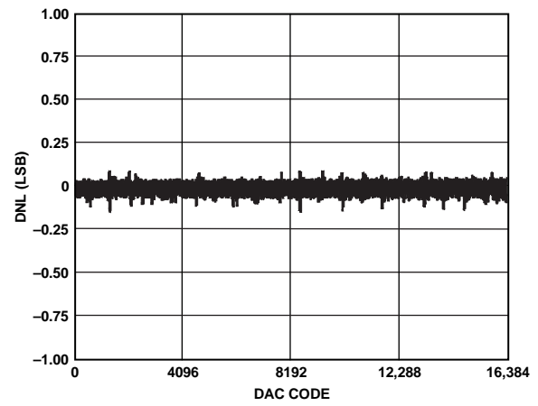
Figure 11. AD5025 DNL
