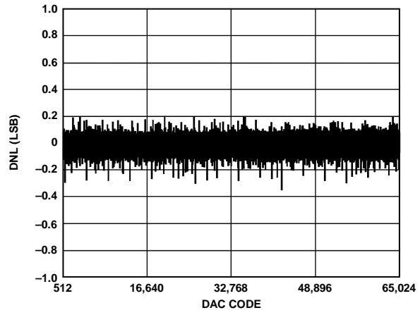
Figure 9. AD5065 DNL
