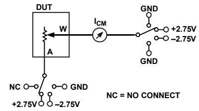
Figure 25. Common Leakage Current
