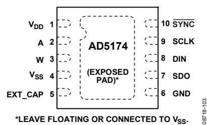
Figure 6. LFCSOP Pin Configuration
