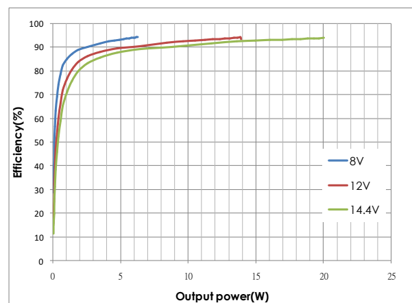
Efficiency (Stereo 8\Omega load) / 2ch
