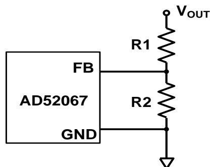
Figure.1 The resistive divider senses the fraction of the output voltage
