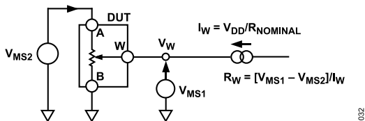
Figure 34. Test Circuit for Wiper Resistance
