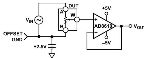
Figure 36. Test Circuit for Gain vs. Frequency
