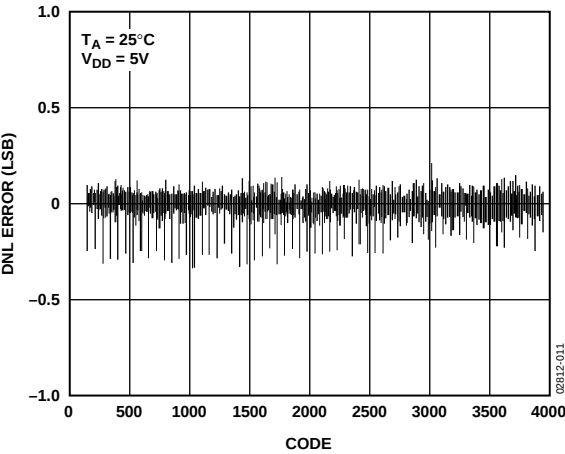
Figure 9. AD5328 Typical DNL Plot
