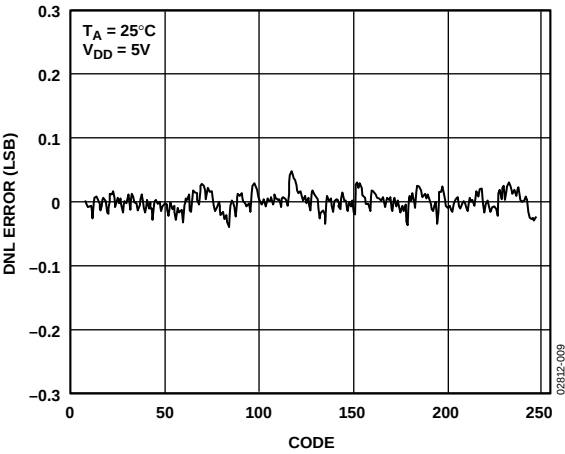
Figure 7. AD5308 Typical DNL Plot
