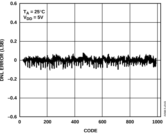
Figure 8. AD5318 Typical DNL Plot
