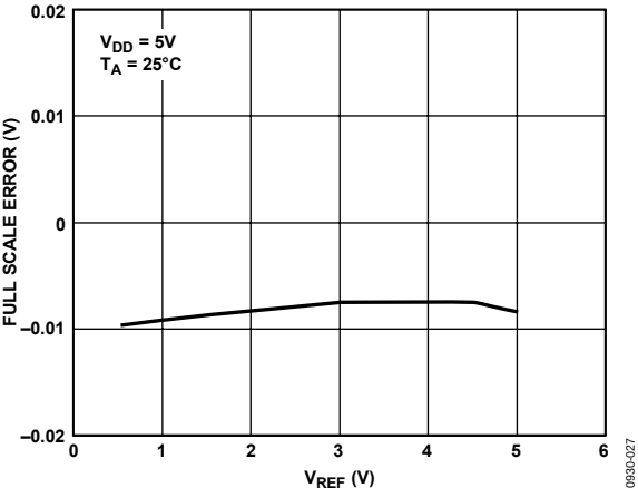
Figure 25. Full-Scale Error vs. V_{REF}
