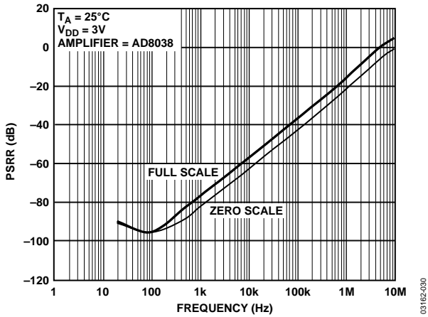
Figure 30. Power Supply Rejection vs. Frequency
