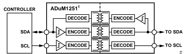
Figure 50. Isolated Interface
