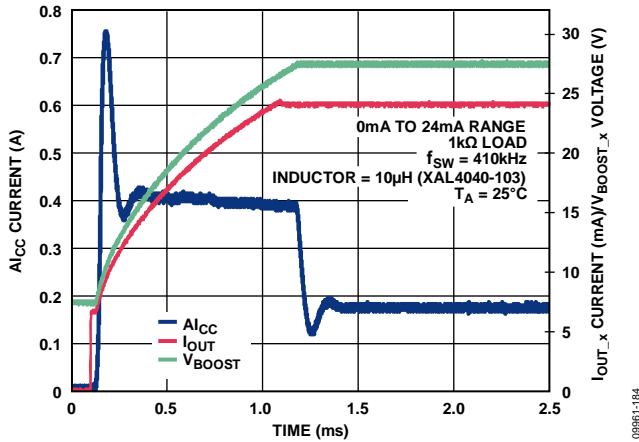
Figure 80. A_{I_{CC}} Current vs. Time for 24 mA Step Through 1 k \Omega Load with Internal Compensation Resistor
