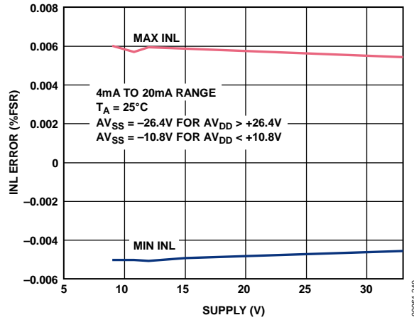
Figure 41. Integral Nonlinearity Error vs. Supply, External R_{SET}
