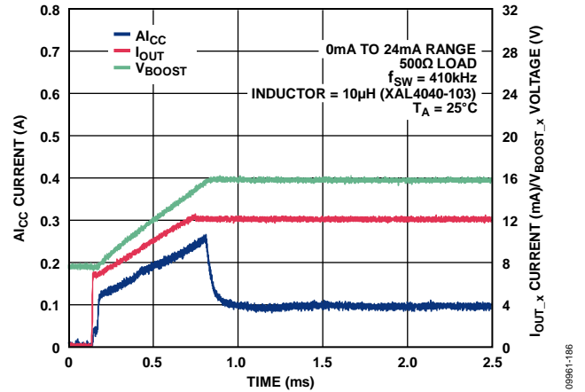
Figure 82. A_{I_{CC}} Current vs. Time for 24 mA Step Through 500 \Omega Load with External 51 k \Omega Compensation Resistor
