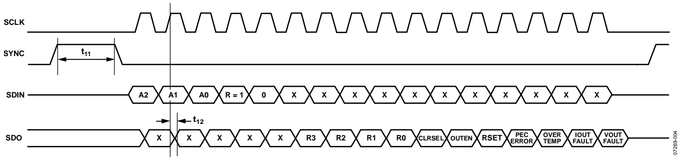
Figure 3. Readback Mode Timing Diagram
