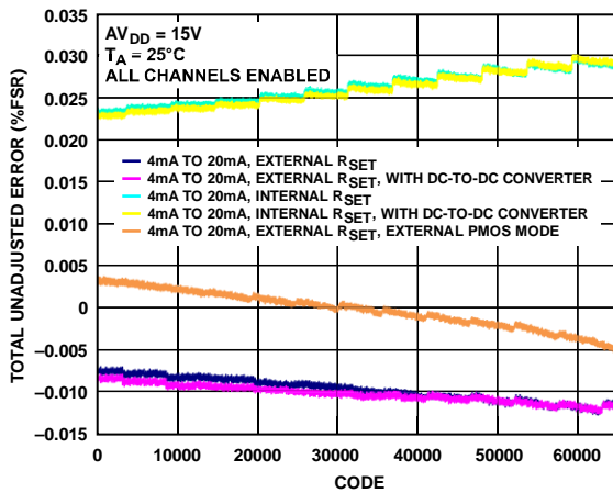
Figure 11. Total Unadjusted Error vs. Code
