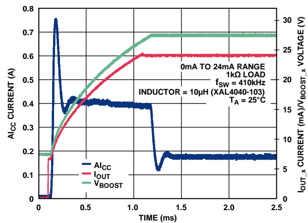
Figure 59. A_{\text{ICC}} Current vs. Time for 24 mA Step Through 1 k \Omega Load with Internal Compensation Resistor
